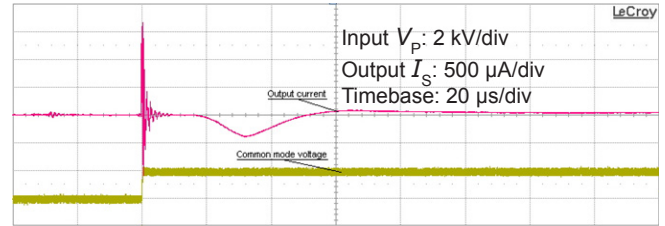
Figure 12: Detail of typical common mode perturbation (2000 V step with 6 kV/µs, R_M = 100 \Omega )
