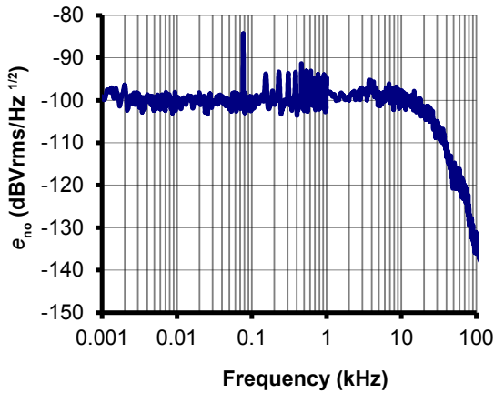
Figure 13: Typical noise voltage density of e_{no} with R_M = 50 \Omega
