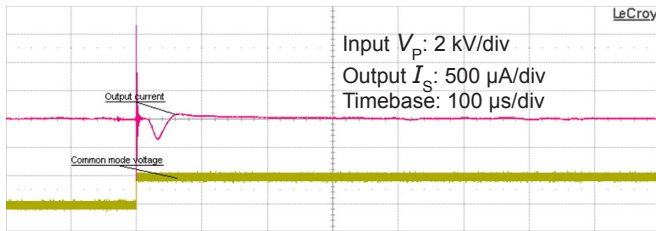
Figure 11: Typical common mode perturbation (2000 V step with 6 kV/µs R_M = 100 \Omega )
