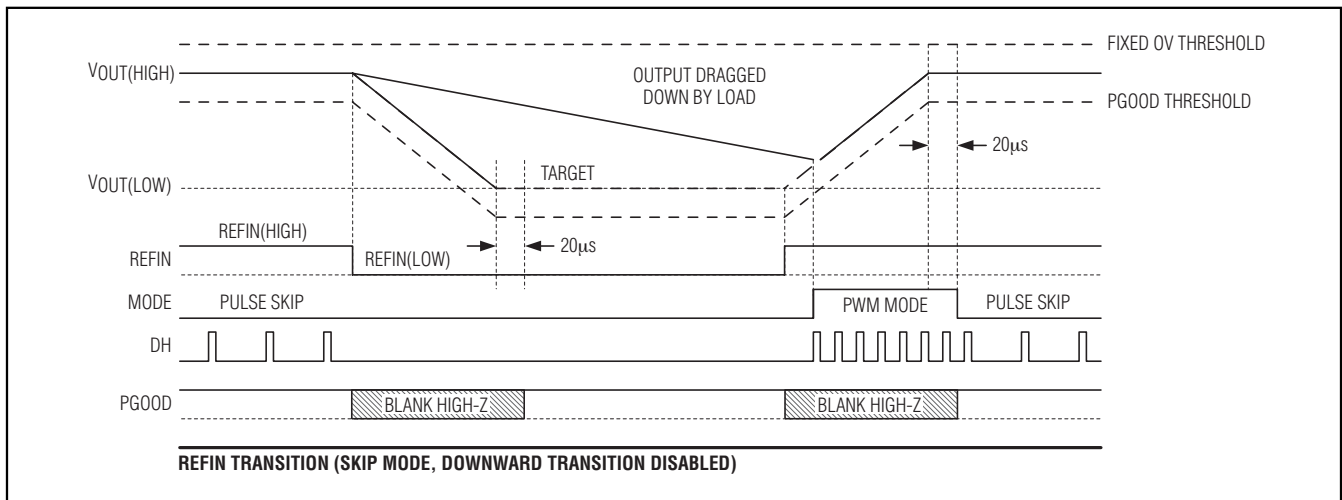
Figure 9. REF IN Transition (Skip Mode, Downward Transition Disabled)
