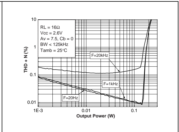
Figure 85. THD+N vs. output power
