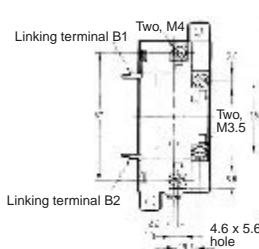
Without Terminal Cover
