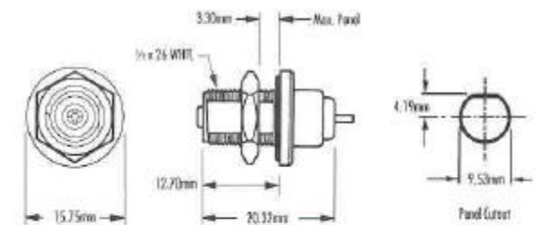
TYPE 142 CONNECTOR FIXED (REAR), STRAIGHT ENTRY, FEMALE CONTACT
