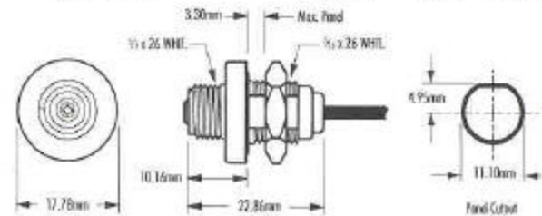
TYPE 132 CONNECTOR FIXED (REAR), STRAIGHT ENTRY, FEMALE CONTACT
