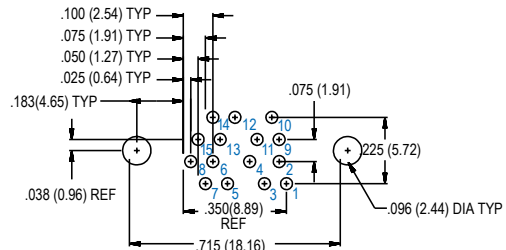
15 PIN
