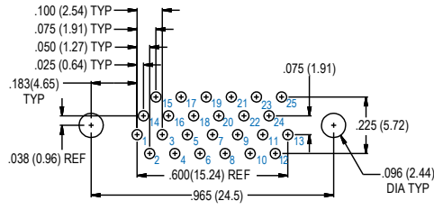
25 SOCKET
