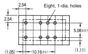
Footprint (Bottom View)
