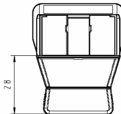
ROW-Stecker/plug 1809281
