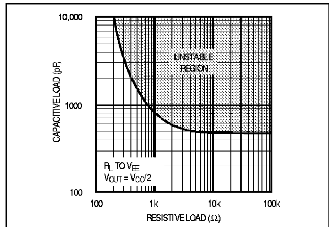
Figure 4. Capacitive-Load Stability
