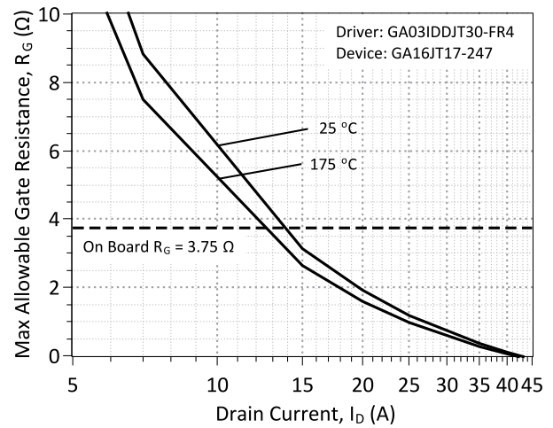
Figure 26: Maximum gate resistance for safe operation of the GA16JT17-247 at different drain currents using the GA03IDDJT30-FR4 board.
