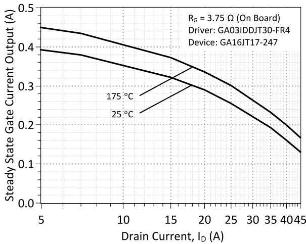
Figure 25: Typical steady state gate current supplied by the GA03IDDJT30-FR4 board for the GA16JT17-247 with the on board resistance of 3.75 Ω
