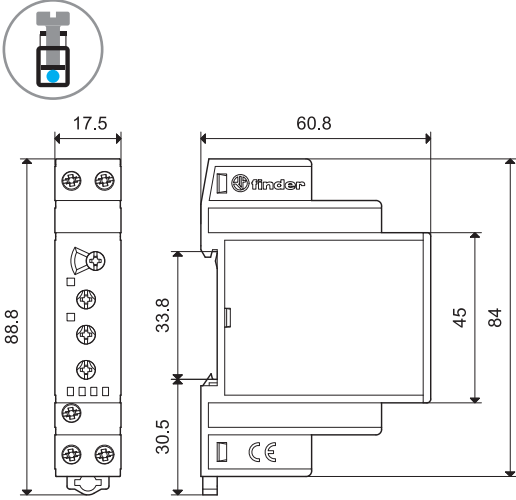
70.11 Screw terminal
