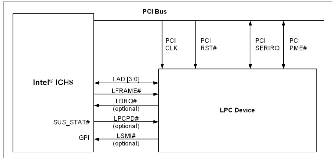
Figure 7. LPC Interface Diagram
