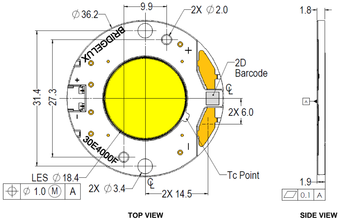
Figure 9: Drawing for Vero 18 LED Array
