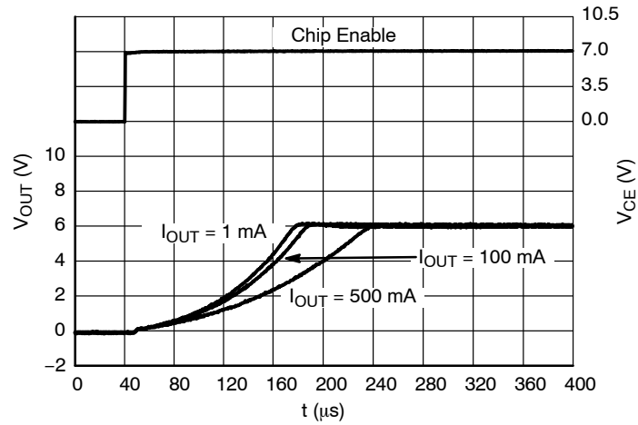
Figure 34. Turn-on Behavior with CE, V_{OUT} = 6 V
