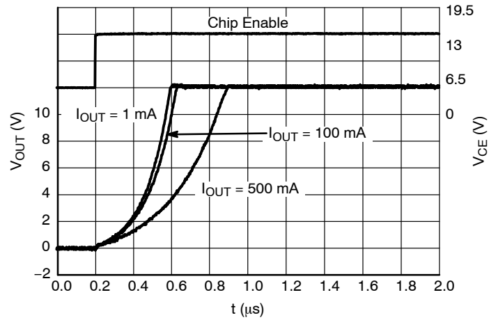
Figure 35. Turn-on Behavior with CE, V_{OUT} = 12 V
