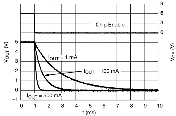
Figure 36. Turn-off Behavior with CE, V_{OUT} = 5 V
