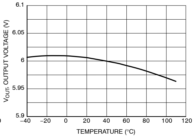
Figure 10. Output Voltage vs. Temperature, V_{OUT} = 6\text{ V}
