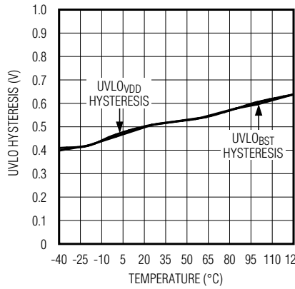
V_{DD} AND BST UNDERVOLTAGE LOCKOUT HYSTERESIS vs. TEMPERATURE
