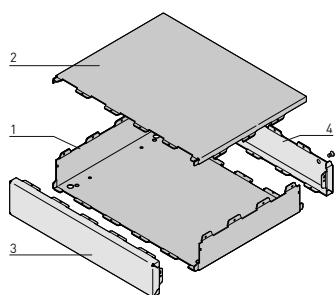
Plain case
