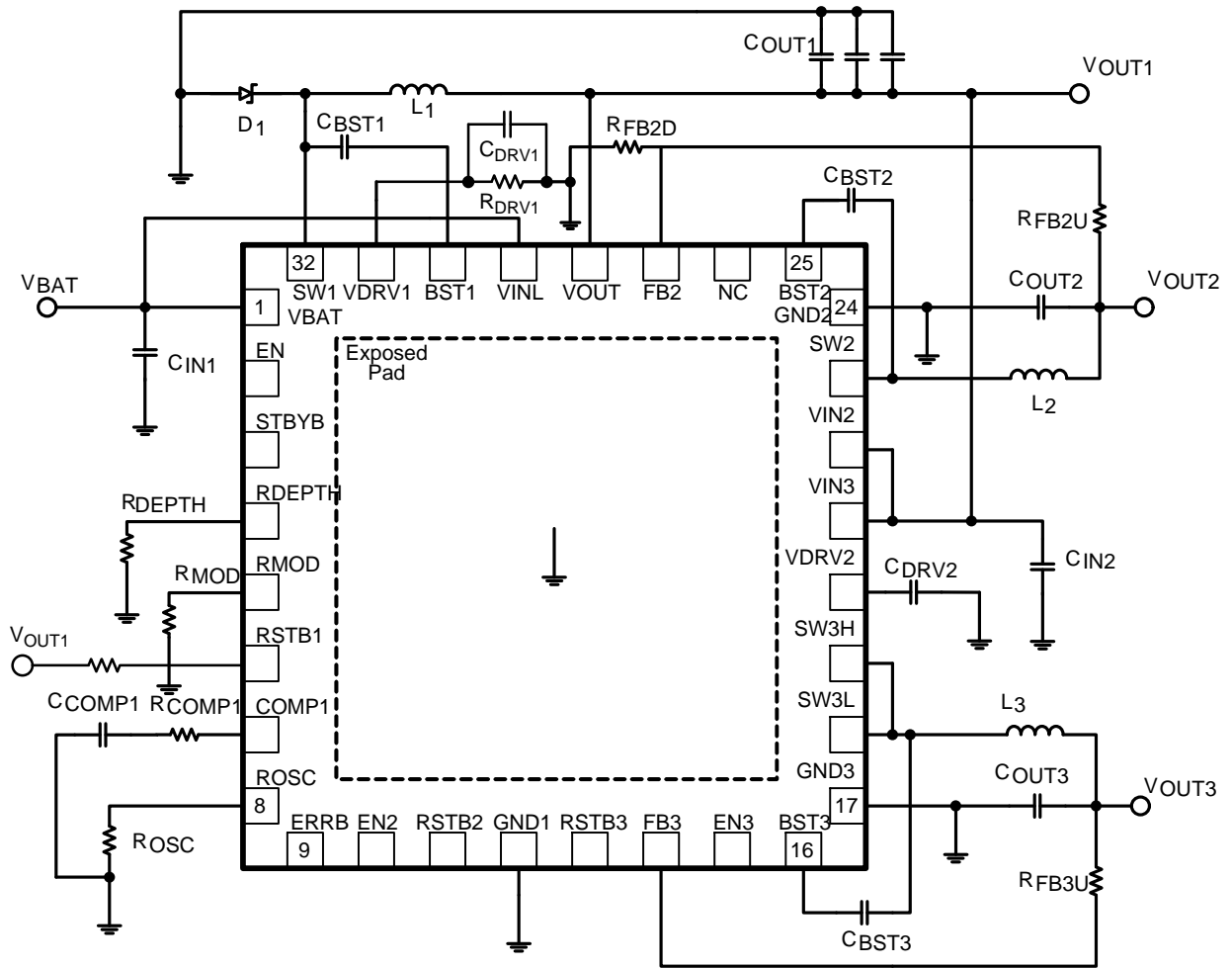
Figure 2. Typical Application
