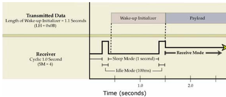
Figure 3-07. Incorrect Configuration (LH < SM)
