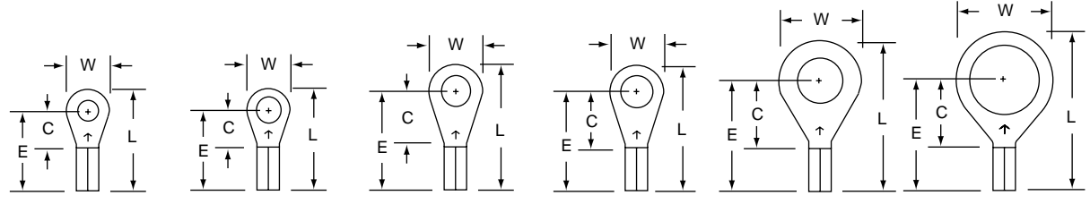
MU18-4R/S MU18-6R/S MU18-8R/L MU18-10R/L MU18-14R/S MU18-38R Stud Size 4 6 8 10 1/4 3/8 Wire Range 22-18 22-18 22-18 22-18 22-18 22-18
