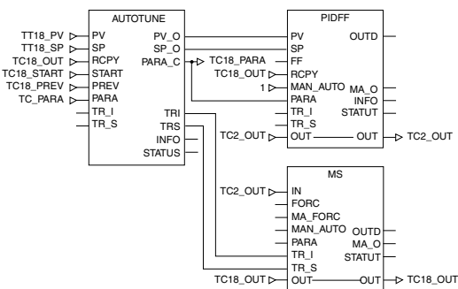
Example: PID controller with MS manual control
