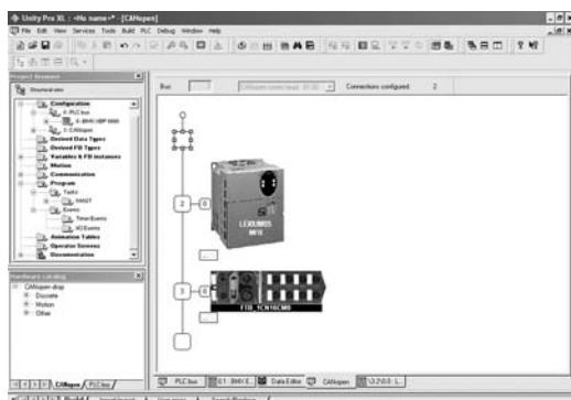
Example of Unity™ Pro configuration screen for Lexium® 05 servo drive and Modicon® FTB IP 67 I/O splitter box
