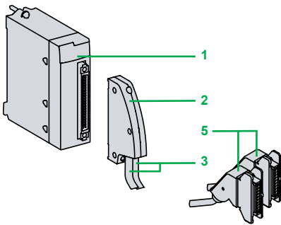
c Preformed cordset with 40-way connector and HE 10 connector for Modicon® Telefast® ABE 7 system
