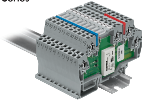
Relay Modules and Optocoupler Modules 859 Series
