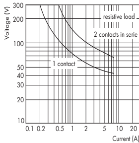
Load limit curve for 788-334 and 788-538
