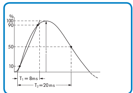
Current pulses 8 /20 per IEC 60060-1/DIN VDE 0432 P. 2
