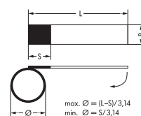
Dimensions of self-laminating label
