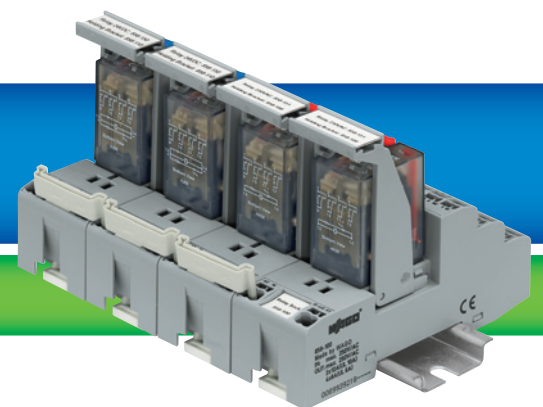
Sockets with Industrial Relay 858 Series
