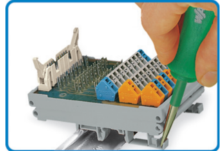
Removal of a module from the carrier rail
