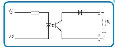
2-wire output
