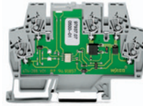
Rail-mounted terminal blocks with optocouplers
