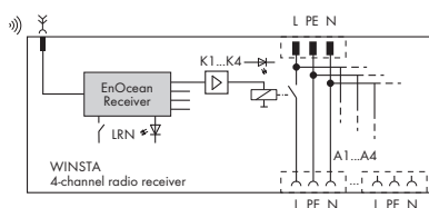
Illustration and block diagram for 770-629/101-000
