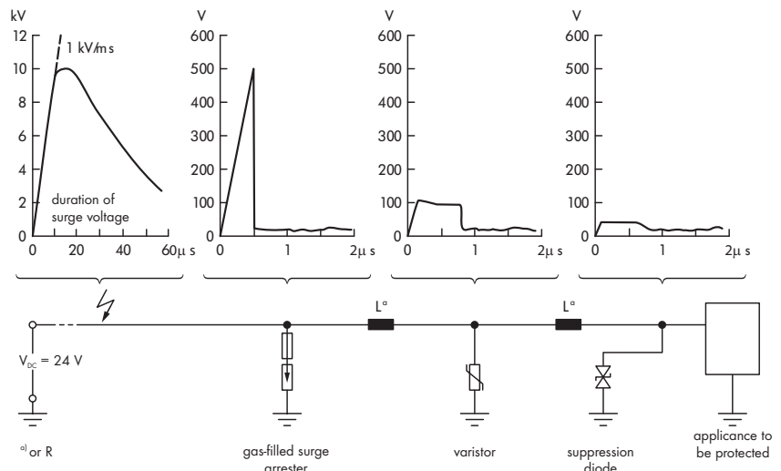
Function diagram of a multi-stage surge voltage protection module
