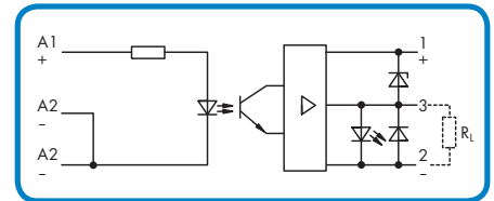
3-wire output positive switching
