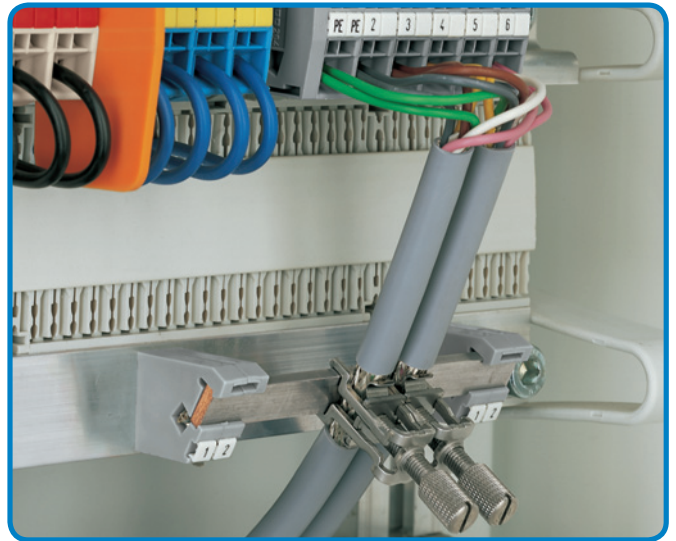
- isolated mounting carriers for a common shield (screen) reference potential, independent of the housing potential
