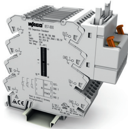
JUMPFLEX® - 8-Channel Adapter 857 Series
