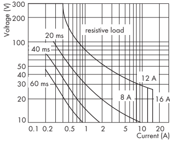
Load limit curve for 788-324 and 788-528
