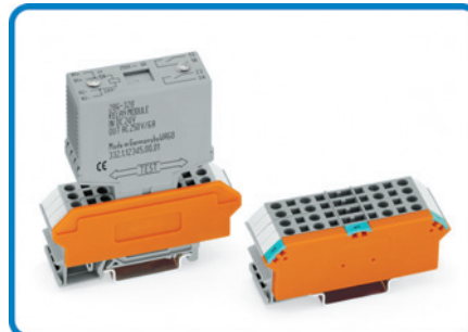
Pluggable function modules
