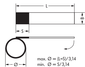
Dimensions of self-laminating label
