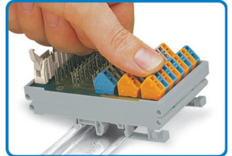
Assembly of a module on the carrier rail
