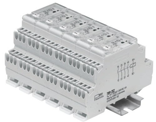
Relay Modules in DIN-Rail Mounted Enclosure 789 Series
