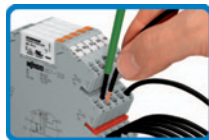
Wire connection
