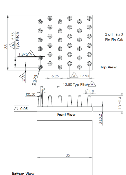
Drawing I: 35x35x10mm
