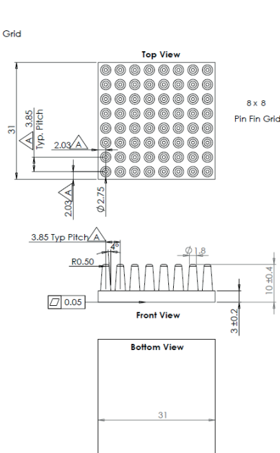
Drawing H: 31x31x10mm
