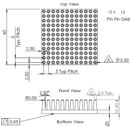
Drawing M: 60x60x15mm
