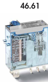
46.61 • 1 Pole CO, 16 A • Plug-in/Faston 187
