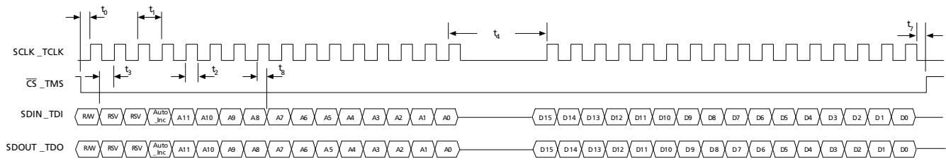
Figure 4-42: Write Mode
