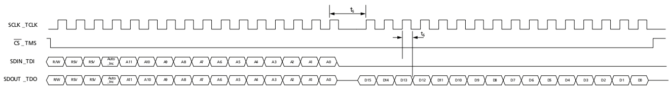
Figure 4-43: Read Mode
