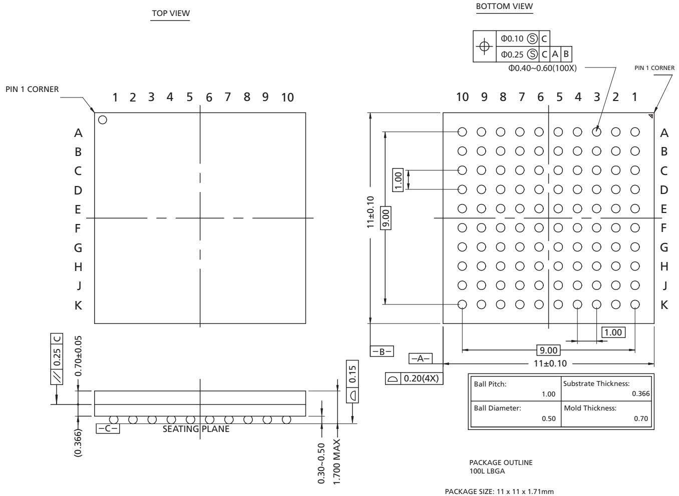
Figure 7-1: GS1671A Packaging Dimensions
