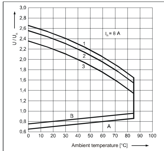
Coil operating range - DC Fig. 4
