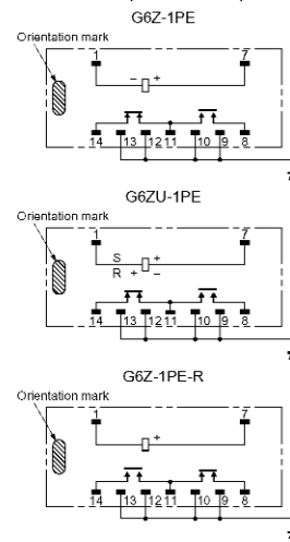
Terminal Arrangement/Internal Connections (Bottom View)
