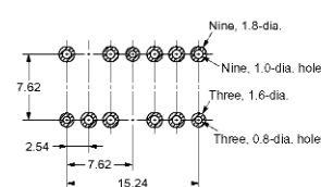
Mounting Dimensions (Bottom View) Tolerance: \pm 0.1 mm
