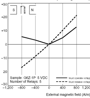
External Magnetic Interference (Average value)
