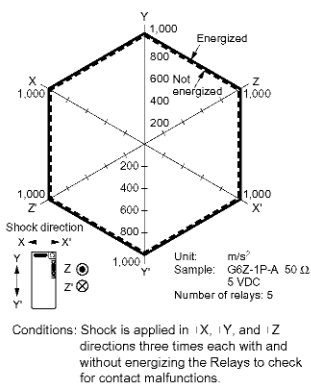
Shock Malfunction
