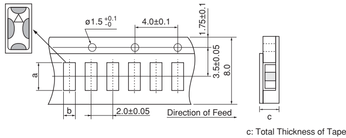
c: Total Thickness of Tape
