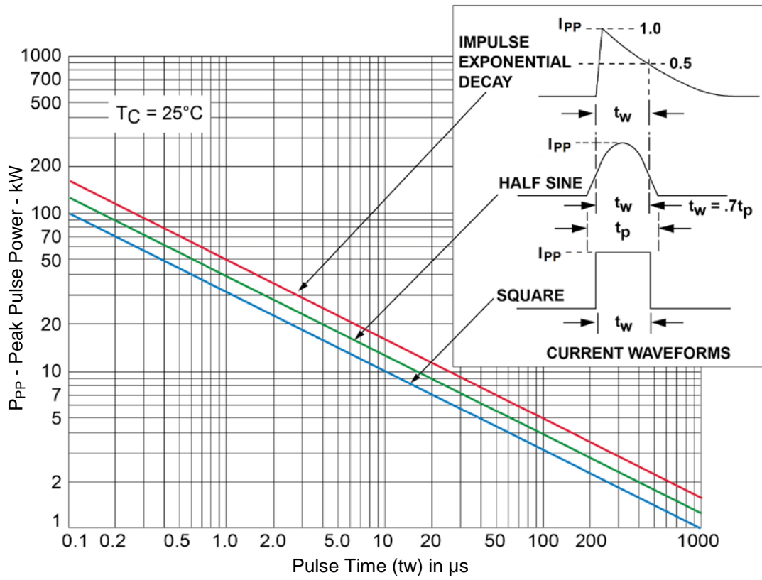
FIGURE 1 Peak Pulse Power vs Pulse Time ( t_w ) in \mu s
