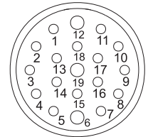
Female insert on plug side
