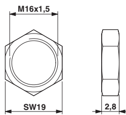
Dimensioned drawing
