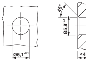
Dimensioned drawing
