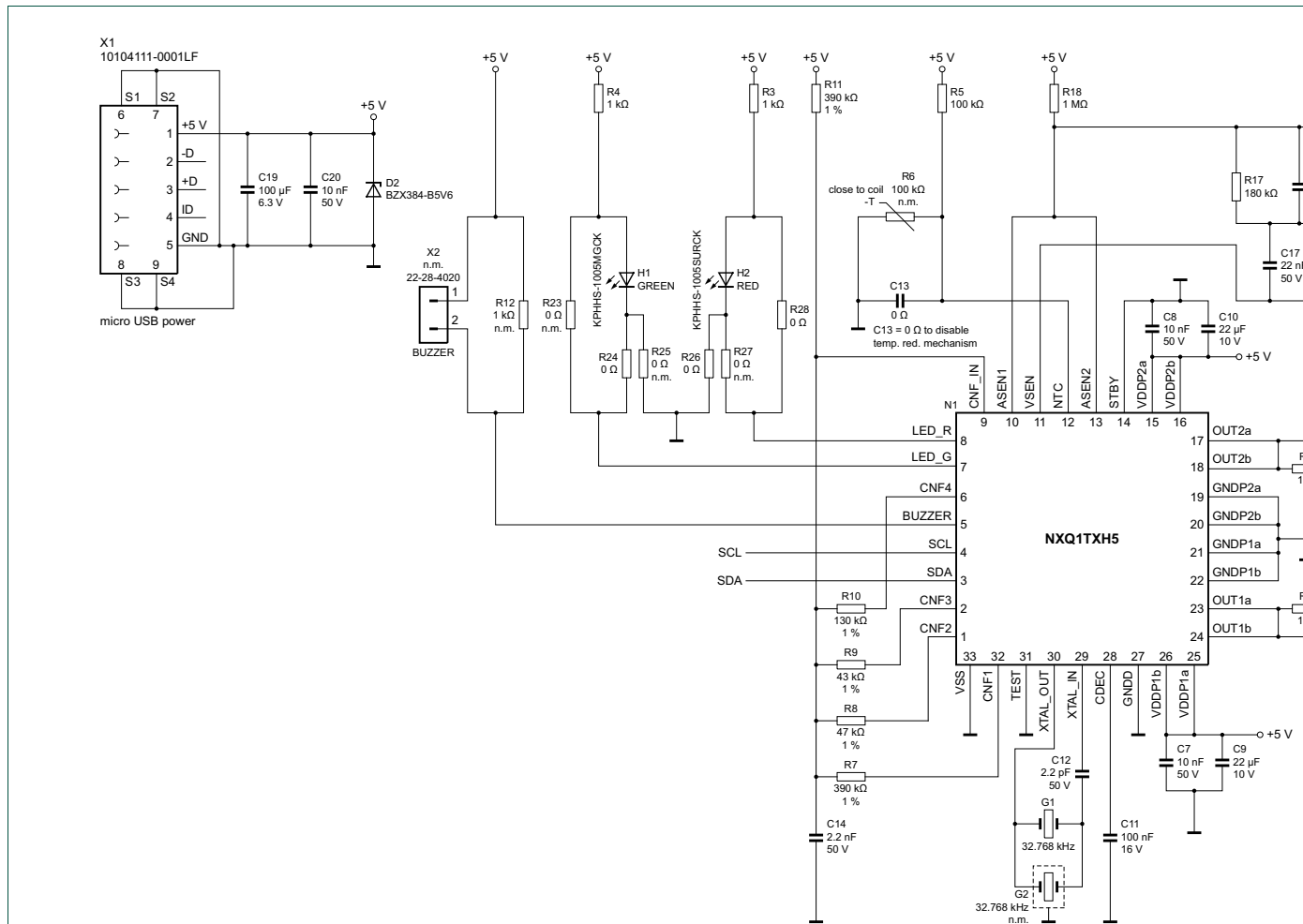
Fig 4. NXQ1TXH5DB1401 demo board schematic diagram
