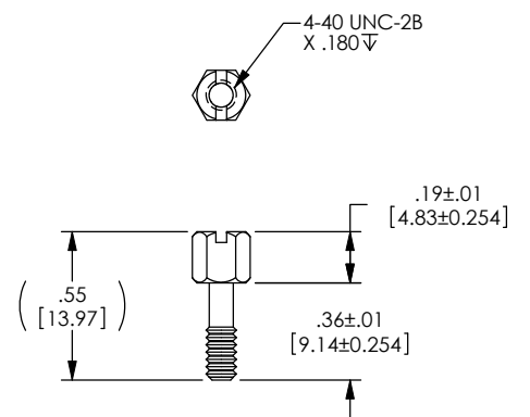
JACKSCREW SPECIFICATION
