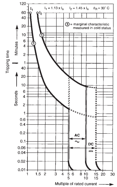
trip characteristic: C I_n = 0.5 \dots 63 \text{ A} S 200/S 200 M MCBs
