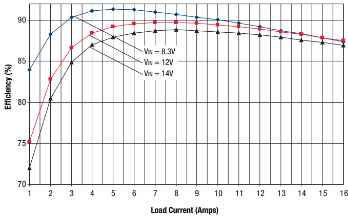
OKX2-T/16-D12 Efficiency vs. Line Voltage and Load Current @ +25°C (V OUT = 1.8V)
