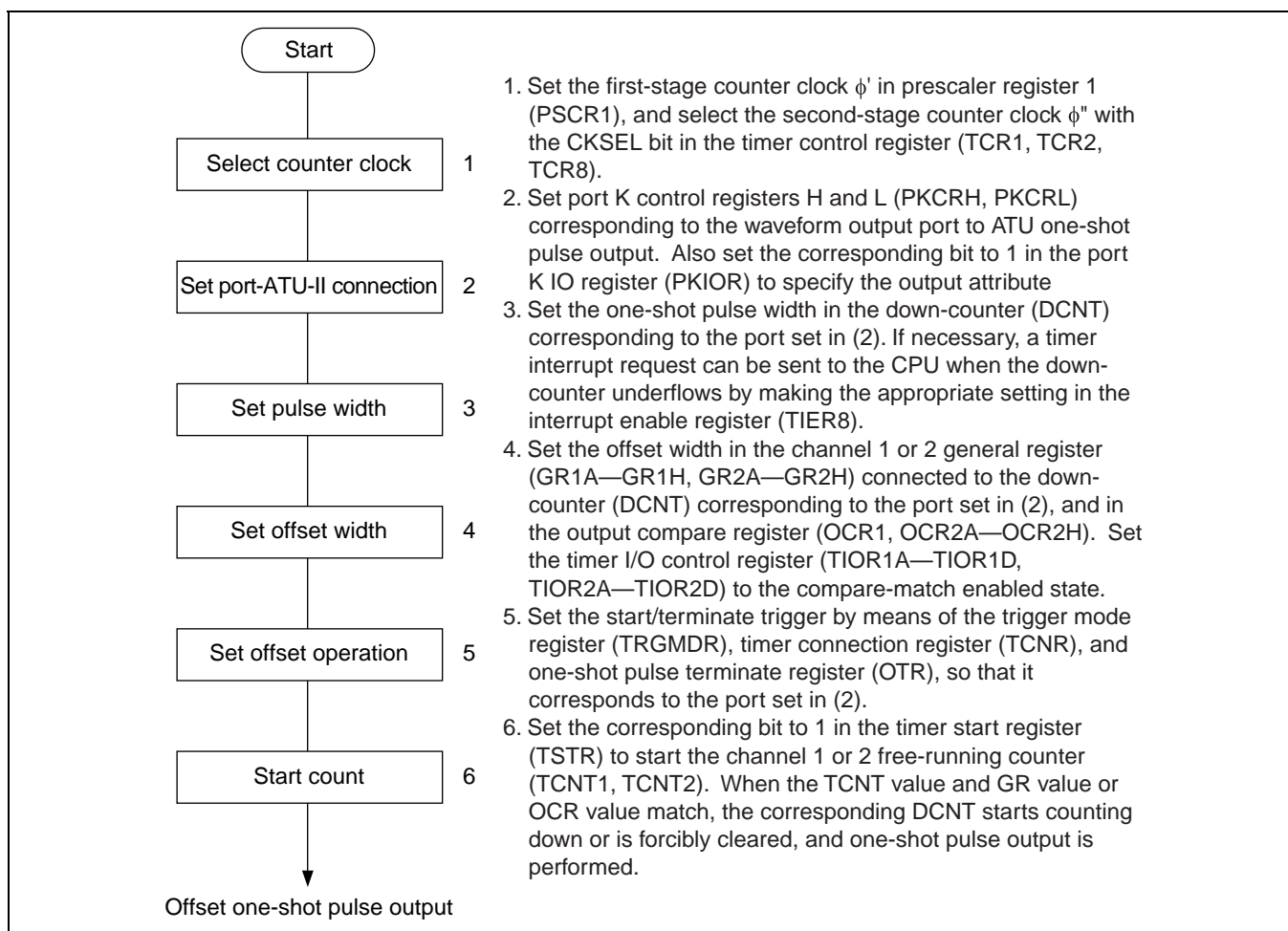
Figure 11.57 Sample Setup Procedure for Offset One-Shot Pulse Output
