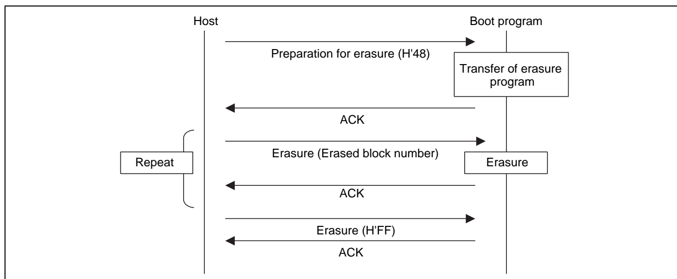
Figure 25.31 Erasing Sequence
