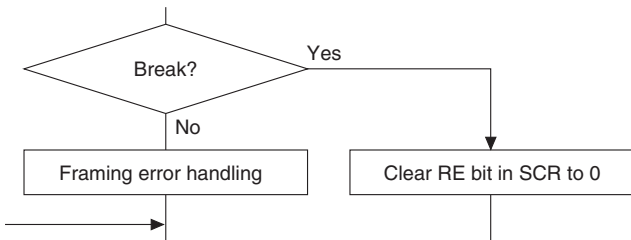
Figure 15.8 Sample Flowchart for Receiving Serial Data (2)
