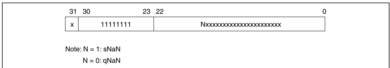
Figure 3.4 NaN Bit Pattern
