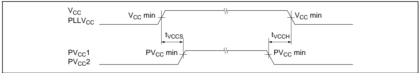
Figure 29.1 Power-On/Off Timing
