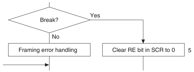
Figure 15.8 Sample Flowchart for Receiving Serial Data (2)
