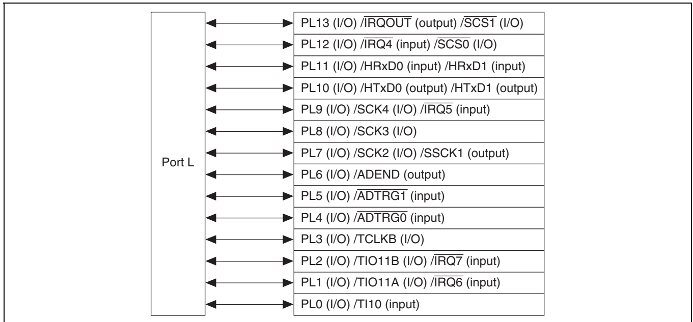
Figure 23.11 Port L
