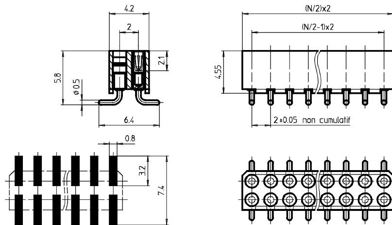
PCB layout
