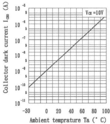
Fig.9 Collector Dark Current vs. Ambient Temperature
