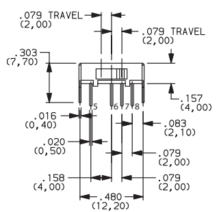
OS203011MA2QP1 DP3T
