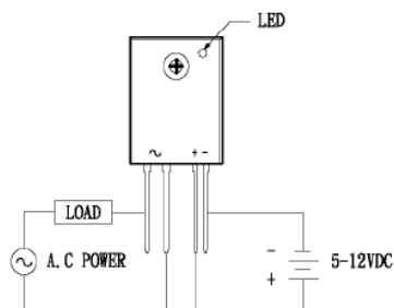
Fig.8 WIRING DIAGRAM
