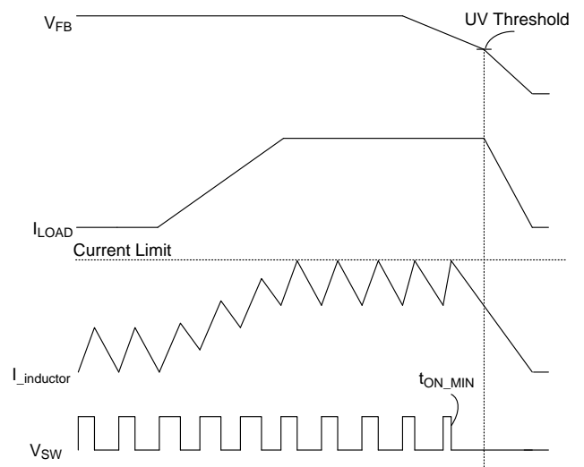
Figure 5. Peak-Current Limit
