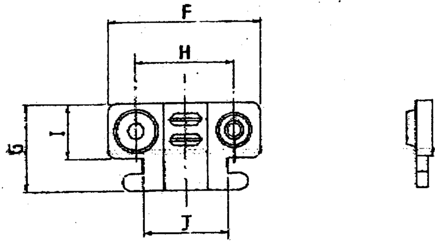
STRAIN RELIEF DETAIL
