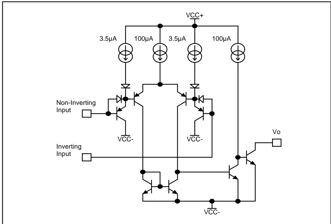
Figure 1: Schematic diagram (1/4 RT2901H)
