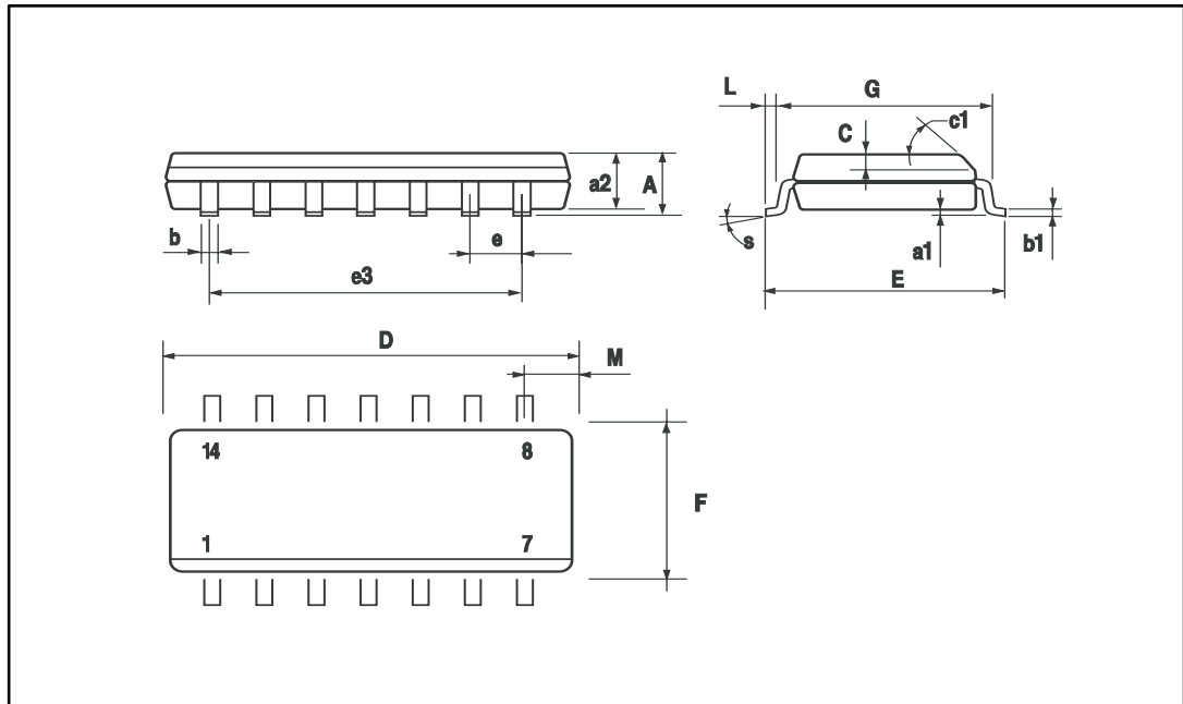
Figure 9: SO14 package mechanical drawing
