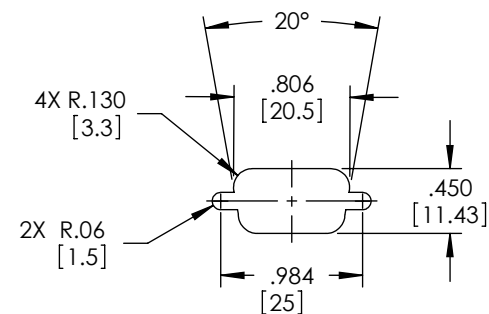
RECOMMENDED PANEL OPENING (MAX PANEL THICKNESS: 0.06")
