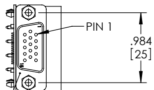
MALE 15 CONTACT HIGH DENSITY D-SUB CONNECTOR
