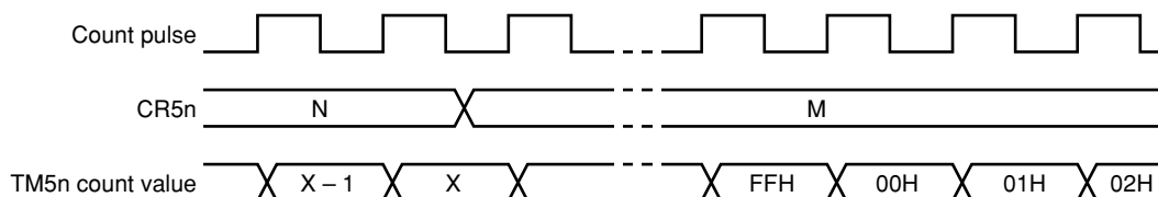
Figure 8-15. Timing After Compare Register Change During Timer Count Operation
