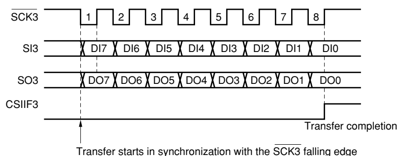
Figure 15-3. Timing of 3-Wire Serial I/O Mode
