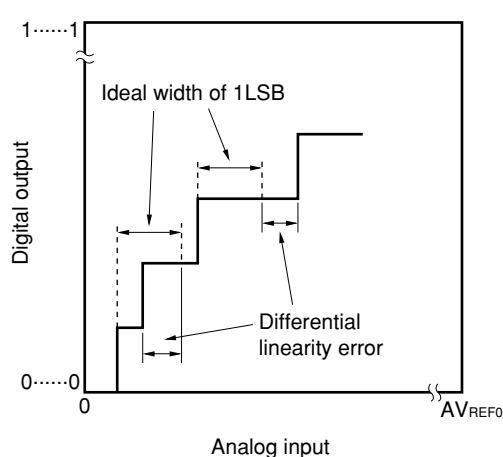
Figure 12-14. Differential Linearity Error
