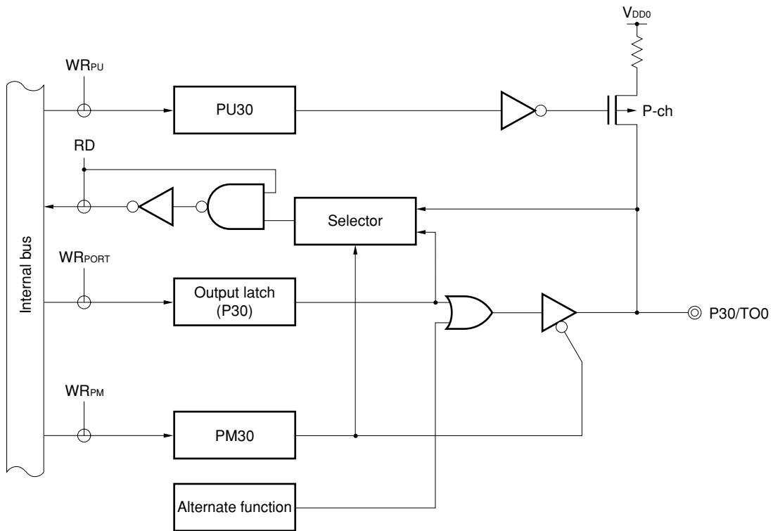
Figure 4-7. P30 Block Diagram
