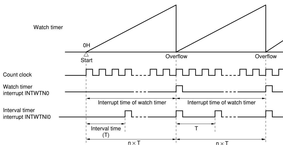
Figure 9-3. Operation Timing of Watch Timer/Interval Timer
