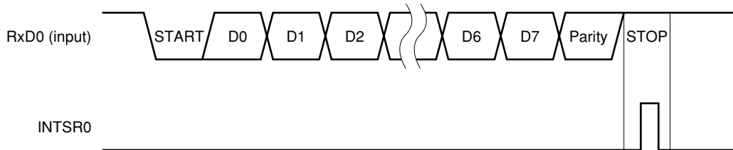
Figure 14-9. Timing of Asynchronous Serial Interface Receive Completion Interrupt Request
