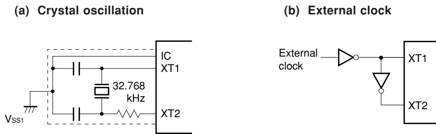
Figure 5-5. External Circuit of Subsystem Clock Oscillator
