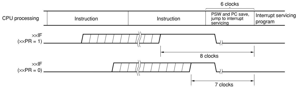
Figure 18-11. Interrupt Request Acknowledge Timing (Minimum Time)
