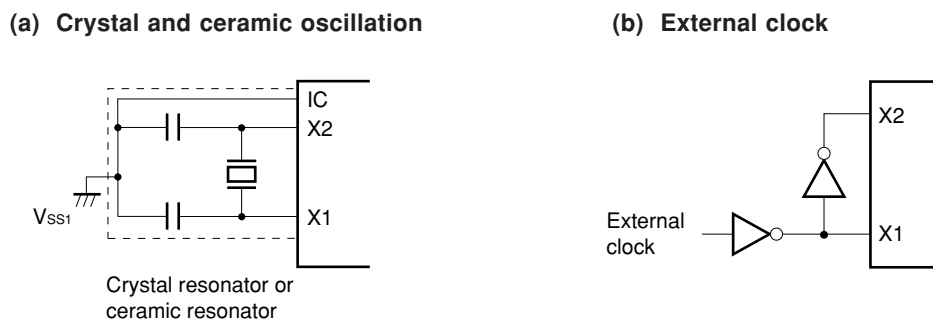
Figure 5-4. External Circuit of Main System Clock Oscillator
