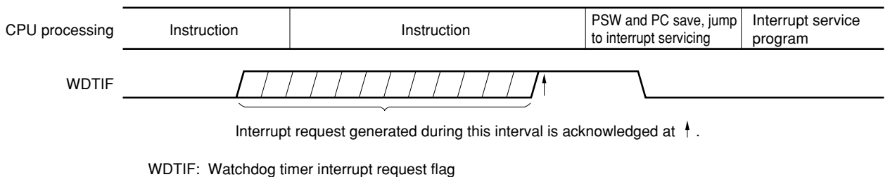
Figure 18-8. Non-Maskable Interrupt Request Acknowledge Timing
