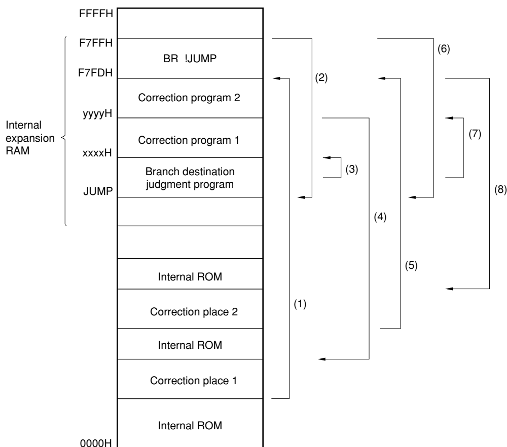
Figure 21-9. Program Transition Diagram (When Two Places Are Corrected)
