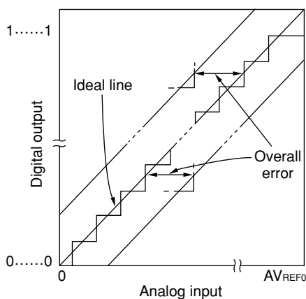
Figure 12-9. Overall Error
