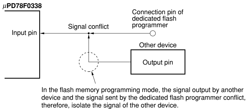
Figure 22-8. Signal Conflict (Input Pin of Serial Interface)
