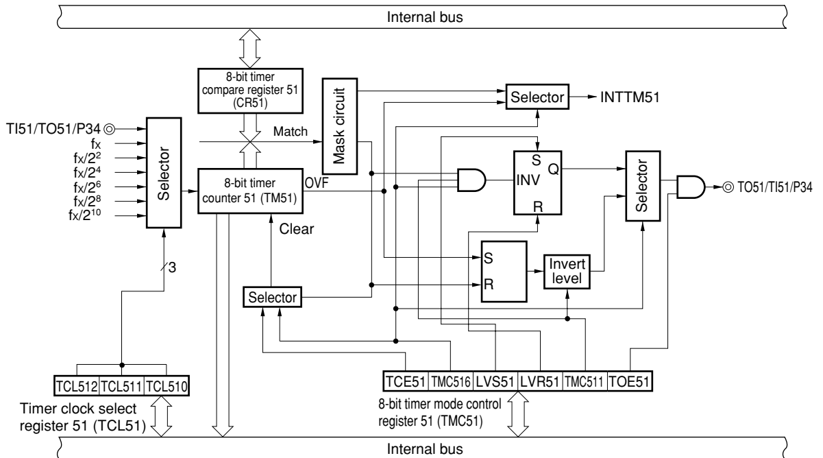
Figure 8-2. 8-Bit Timer/Event Counter 51 Block Diagram
