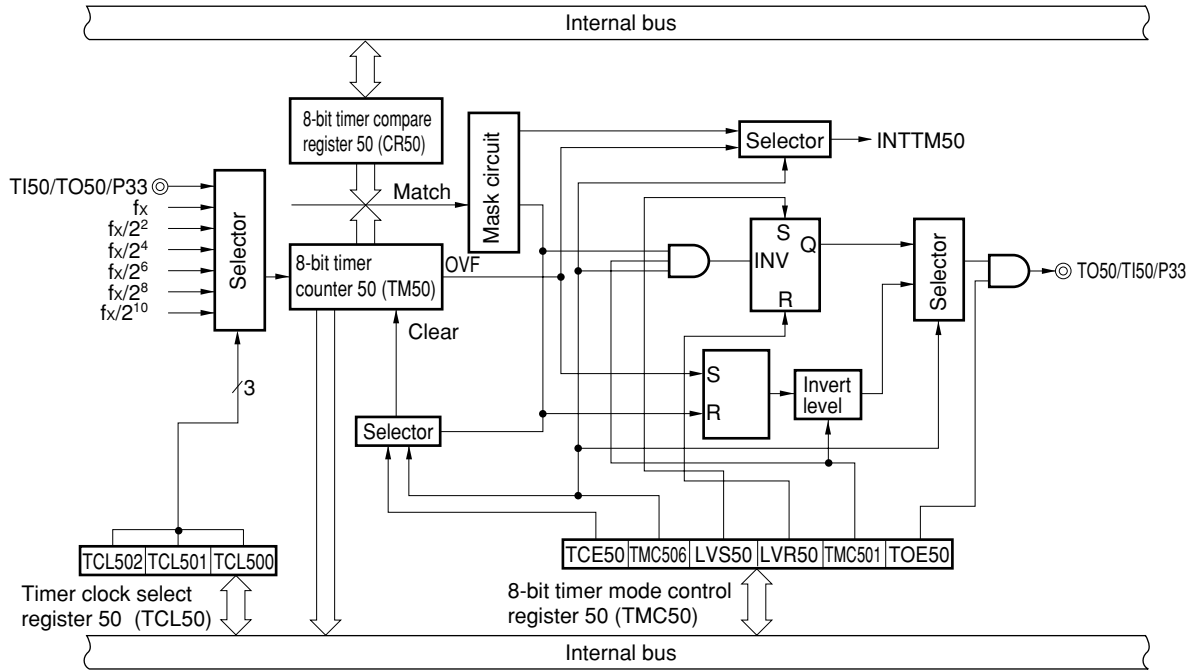
Figure 8-1. 8-Bit Timer/Event Counter 50 Block Diagram
