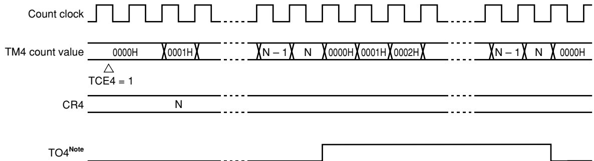
Figure 7-5. Square-Wave Output Operation Timing
