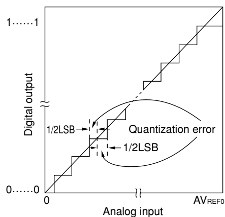
Figure 12-10. Quantization Error
