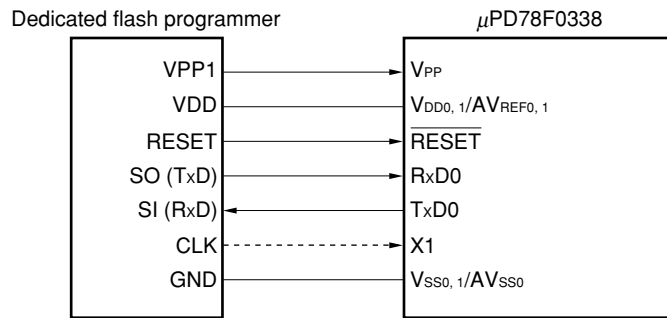
Figure 22-6. UART (UART0)
