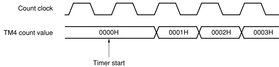
Figure 7-7. 16-Bit Timer Counter 4 (TM4) Start Timing
