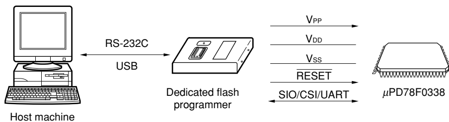
Figure 22-3. Environment for Writing Program to Flash Memory
