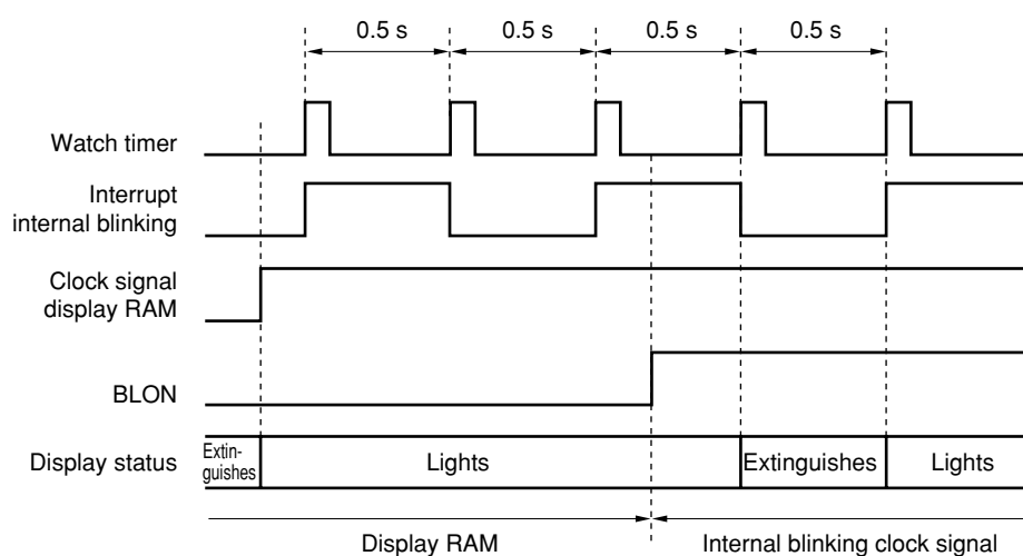
Figure 17-3. Blinking Function
