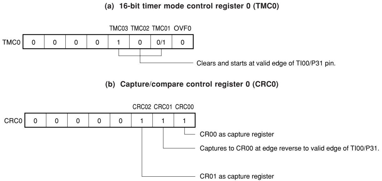
Figure 6-19. Control Register Settings for Pulse Width Measurement by Means of Restart
