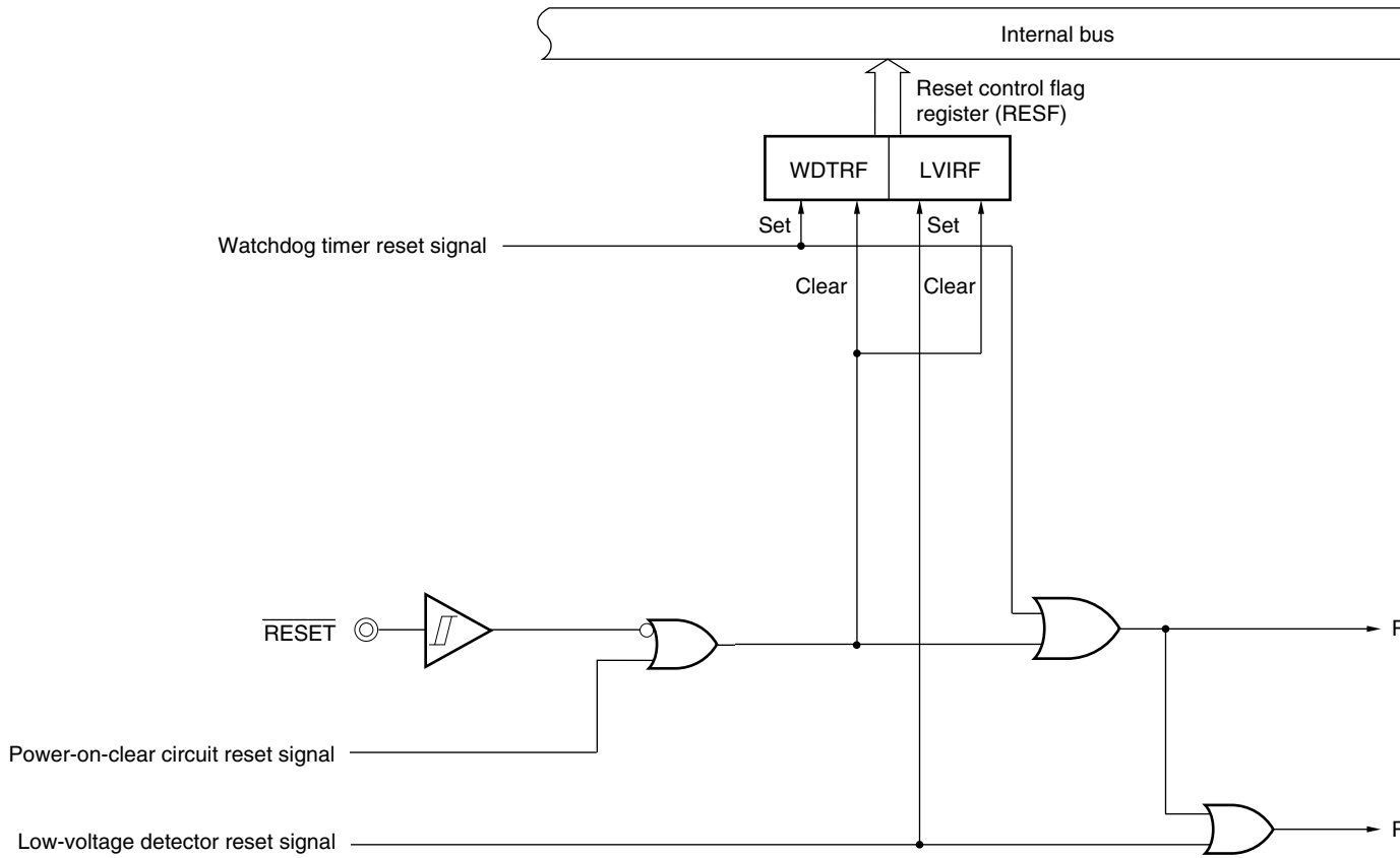
Figure 23-1. Block Diagram of Reset Function
