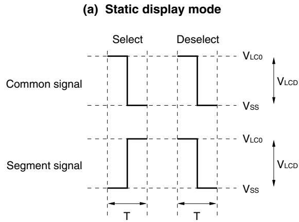
Figure 17-14. Voltages and Phases of Common and Segment Signals
