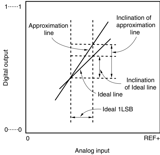
Figure 13-18. Gain Error
