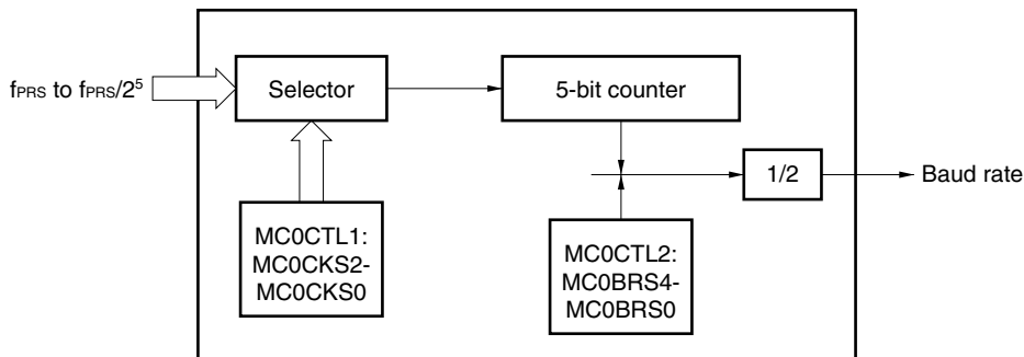
Figure 18-2. Block Diagram of Baud Rate Generator
