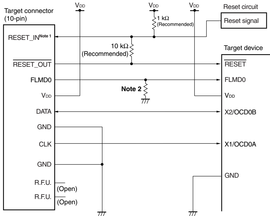
Figure 28-1. Connection Example of QB-MINI2 and 78K0/LE3
