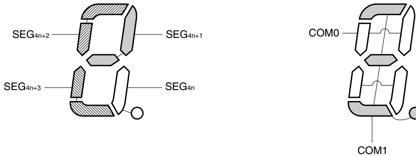
Figure 17-20. Two-Time-Slice LCD Display Pattern and Electrode Connections
