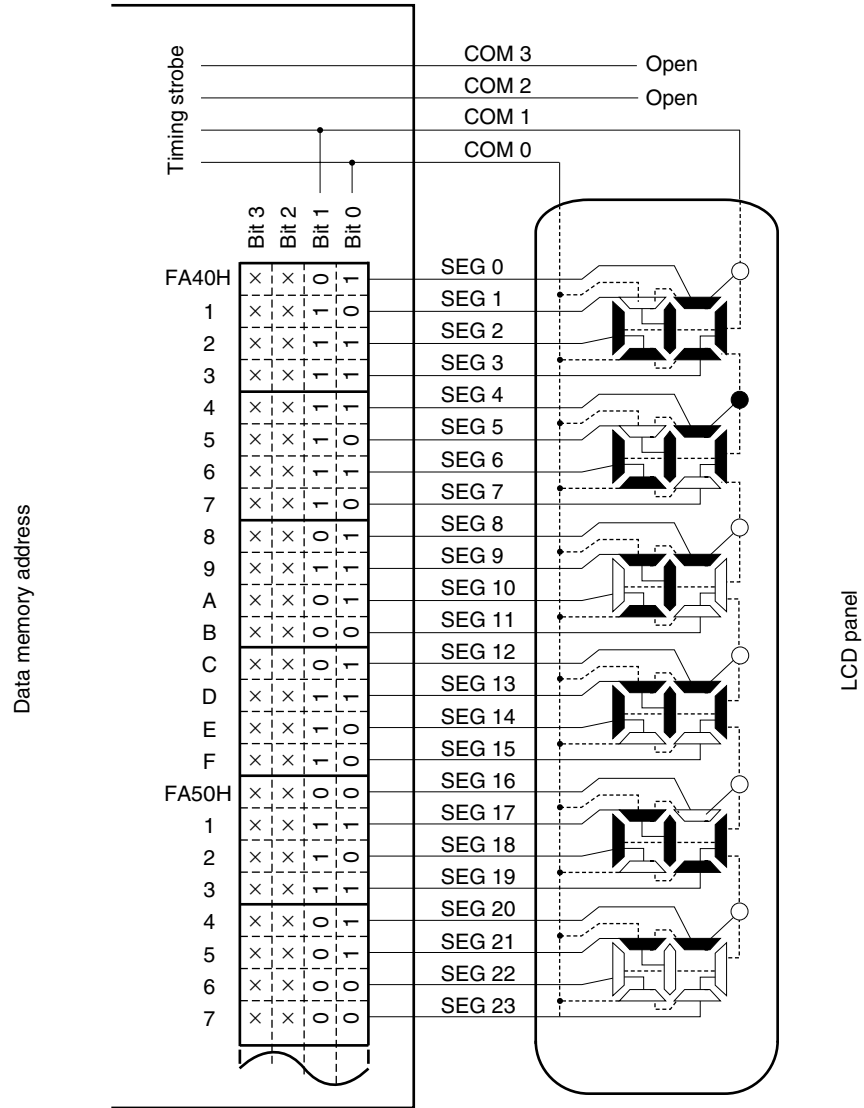
Figure 17-21. Example of Connecting Two-Time-Slice LCD Panel
