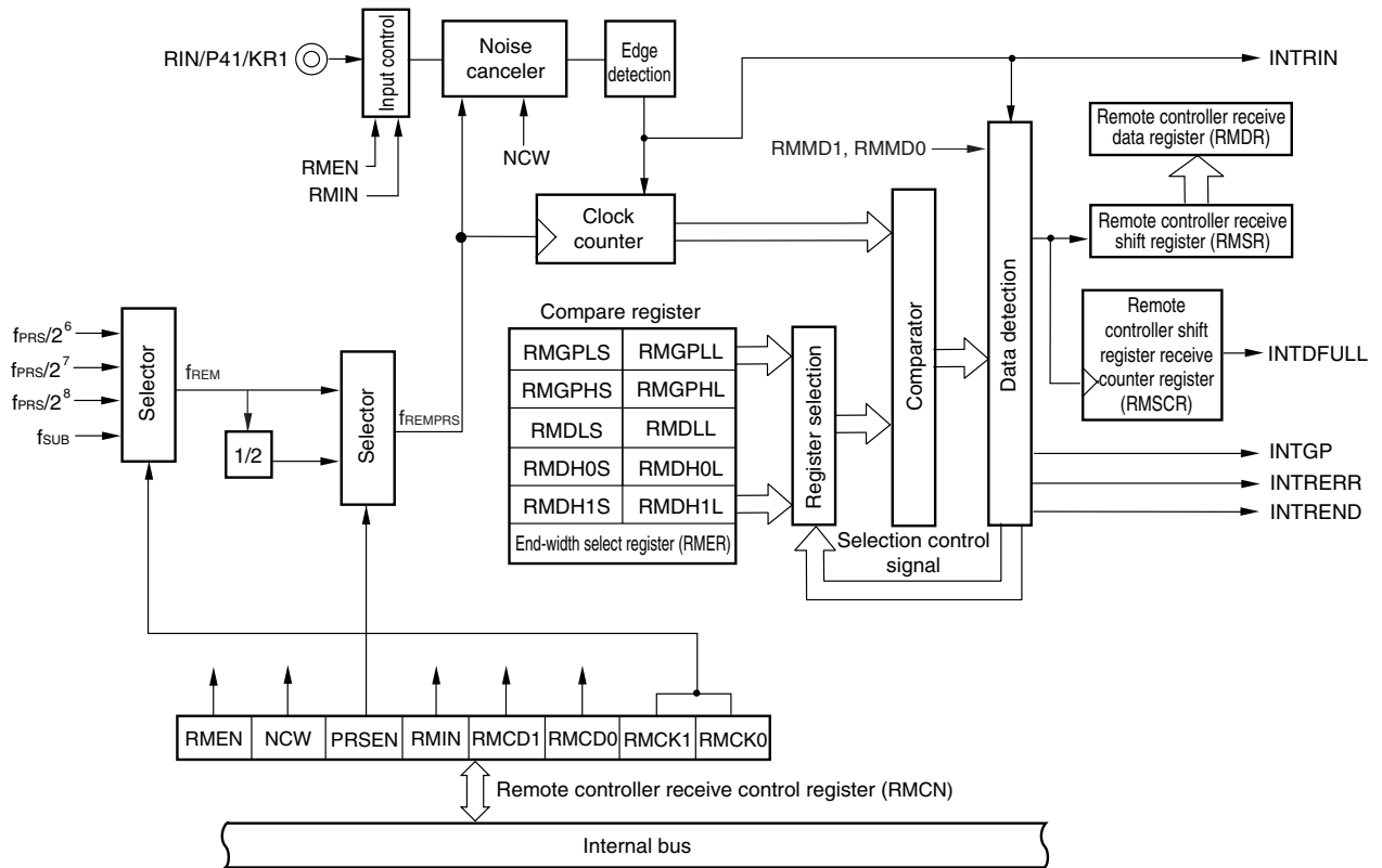
Figure 19-1. Block Diagram of Remote Controller Receiver
