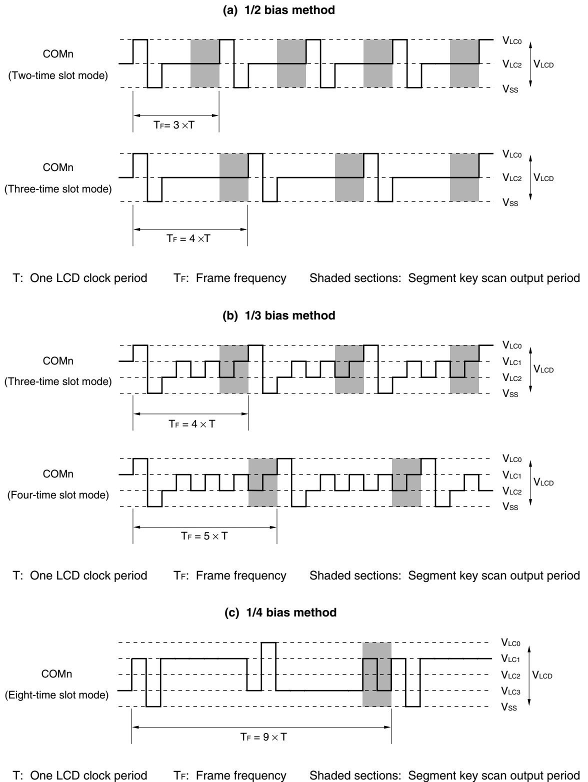
Figure 17-15 Common Signal Waveforms
