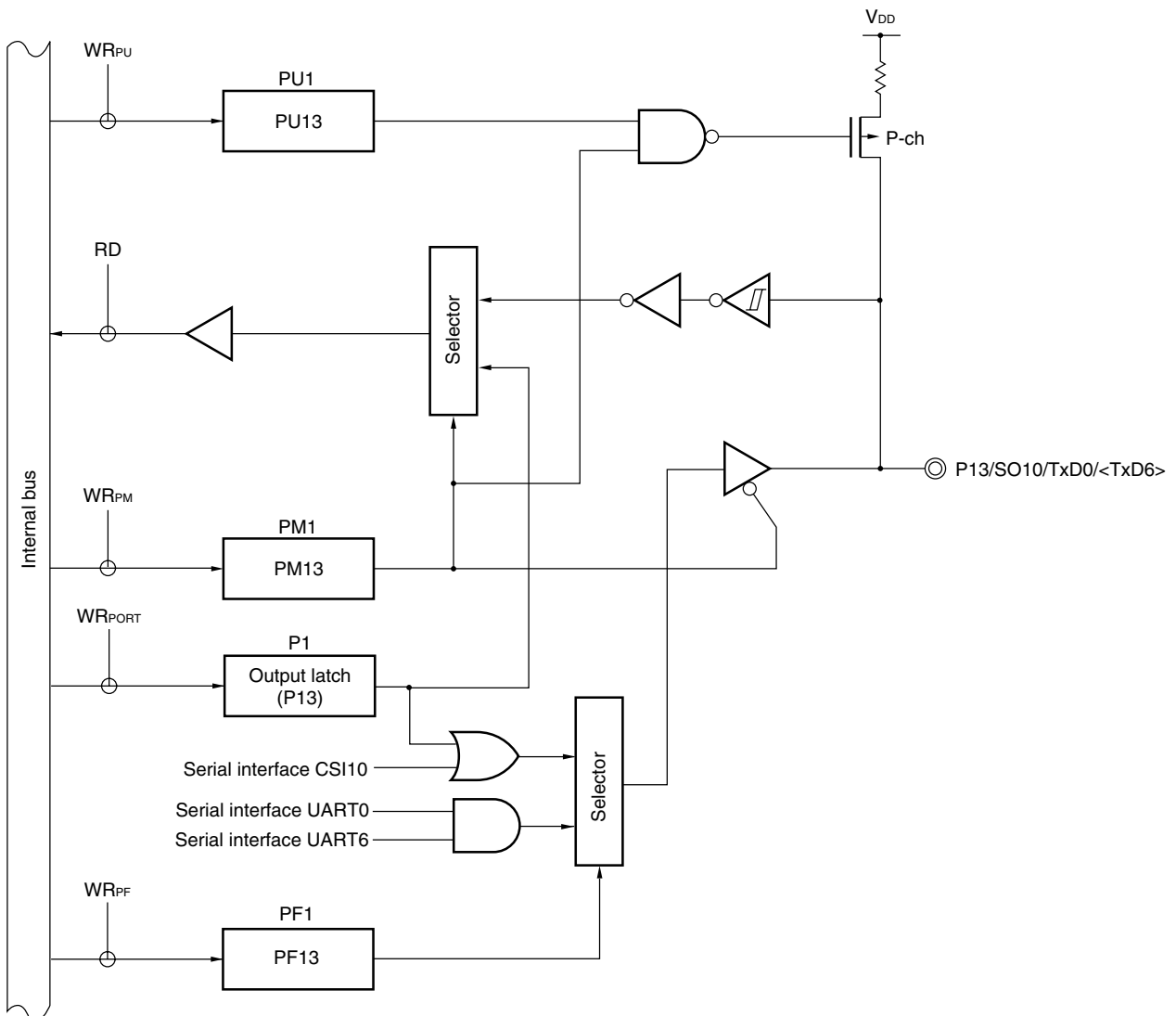
Figure 4-4. Block Diagram of P13
