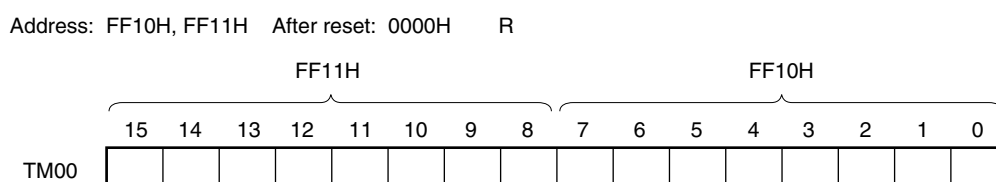
Figure 6-2. Format of 16-Bit Timer Counter 00 (TM00)
