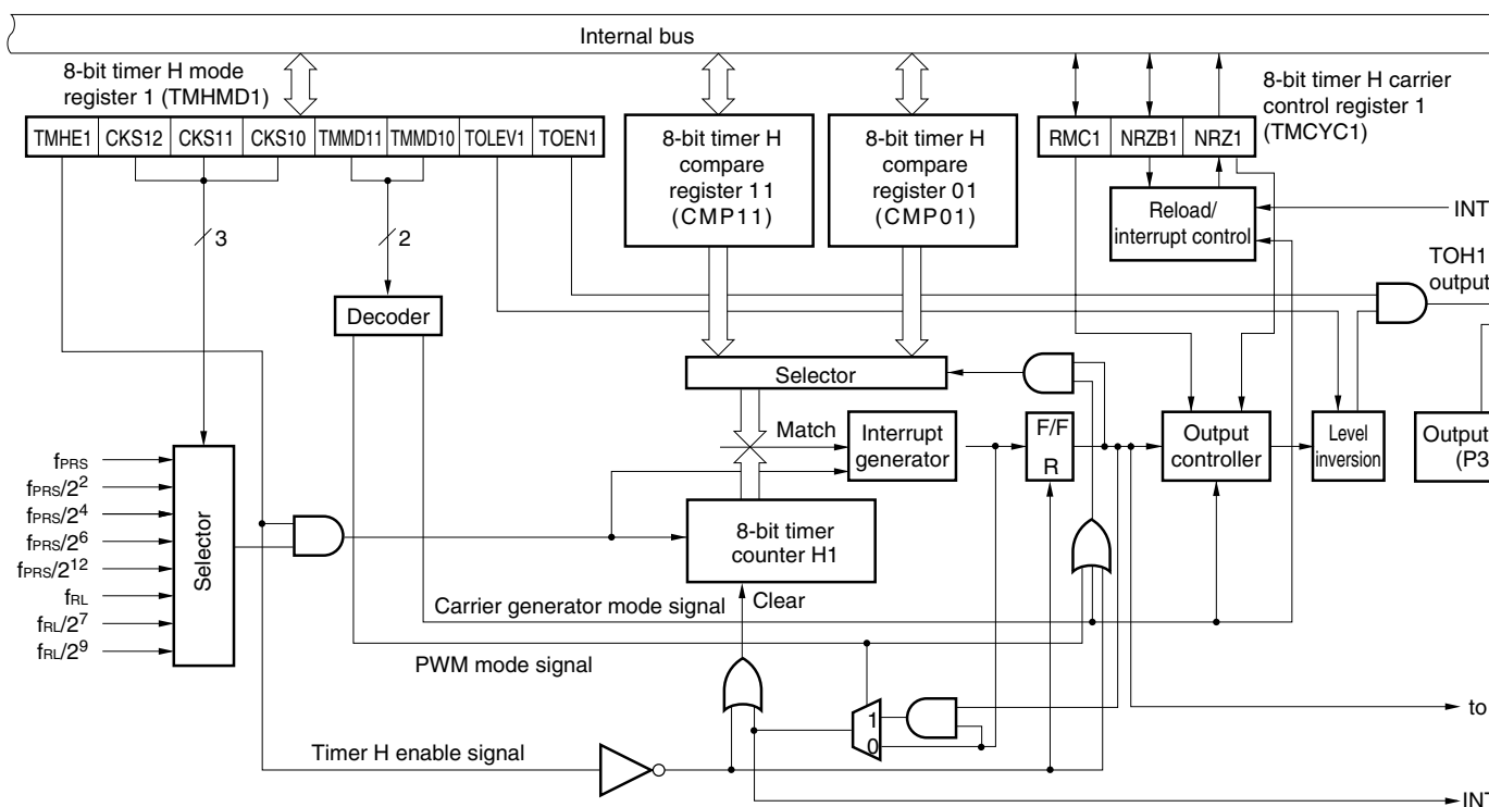
<R> Figure 8-2. Block Diagram of 8-Bit Timer H1
