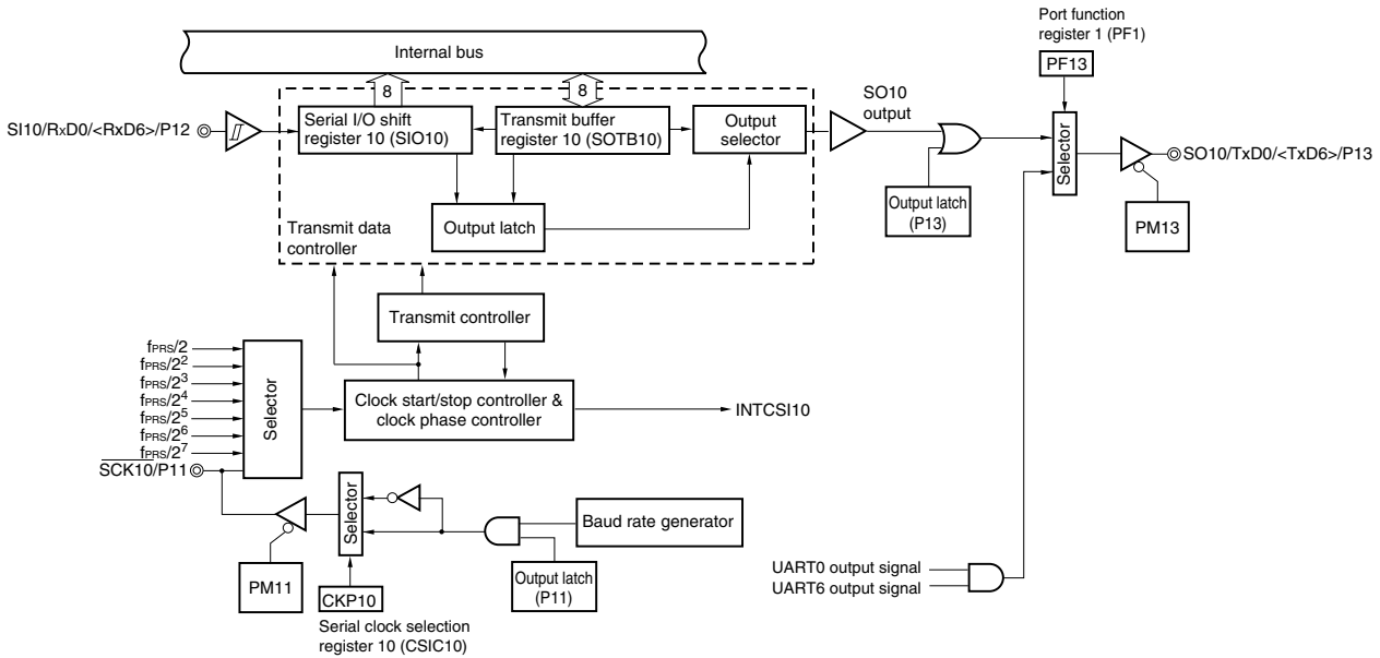
Figure 16-1. Block Diagram of Serial Interface CSI10
