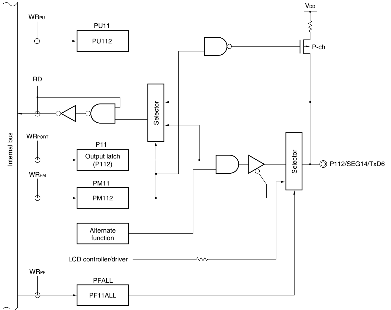
Figure 4-14. Block Diagram of P112
