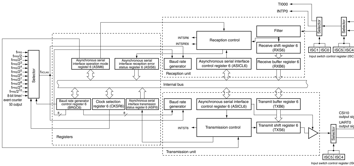
Figure 15-4. Block Diagram of Serial Interface UART6
