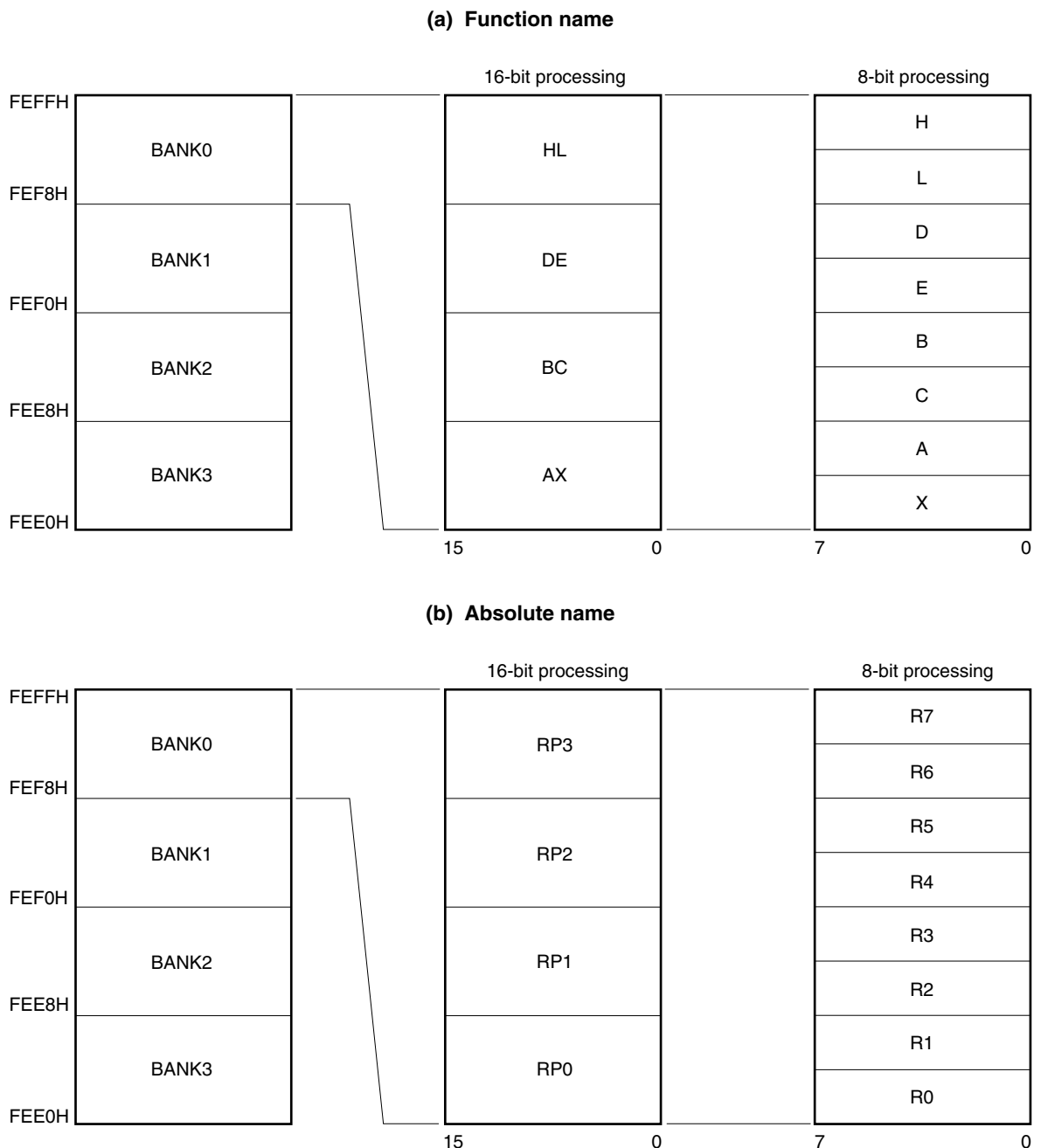
Figure 3-26. Configuration of General-Purpose Registers
