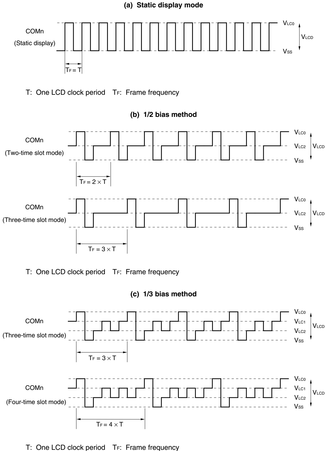
Figure 17-13. Common Signal Waveforms
