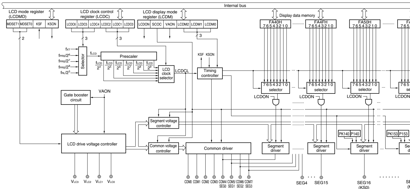
Figure 17-1. Block Diagram of LCD Controller/Driver
