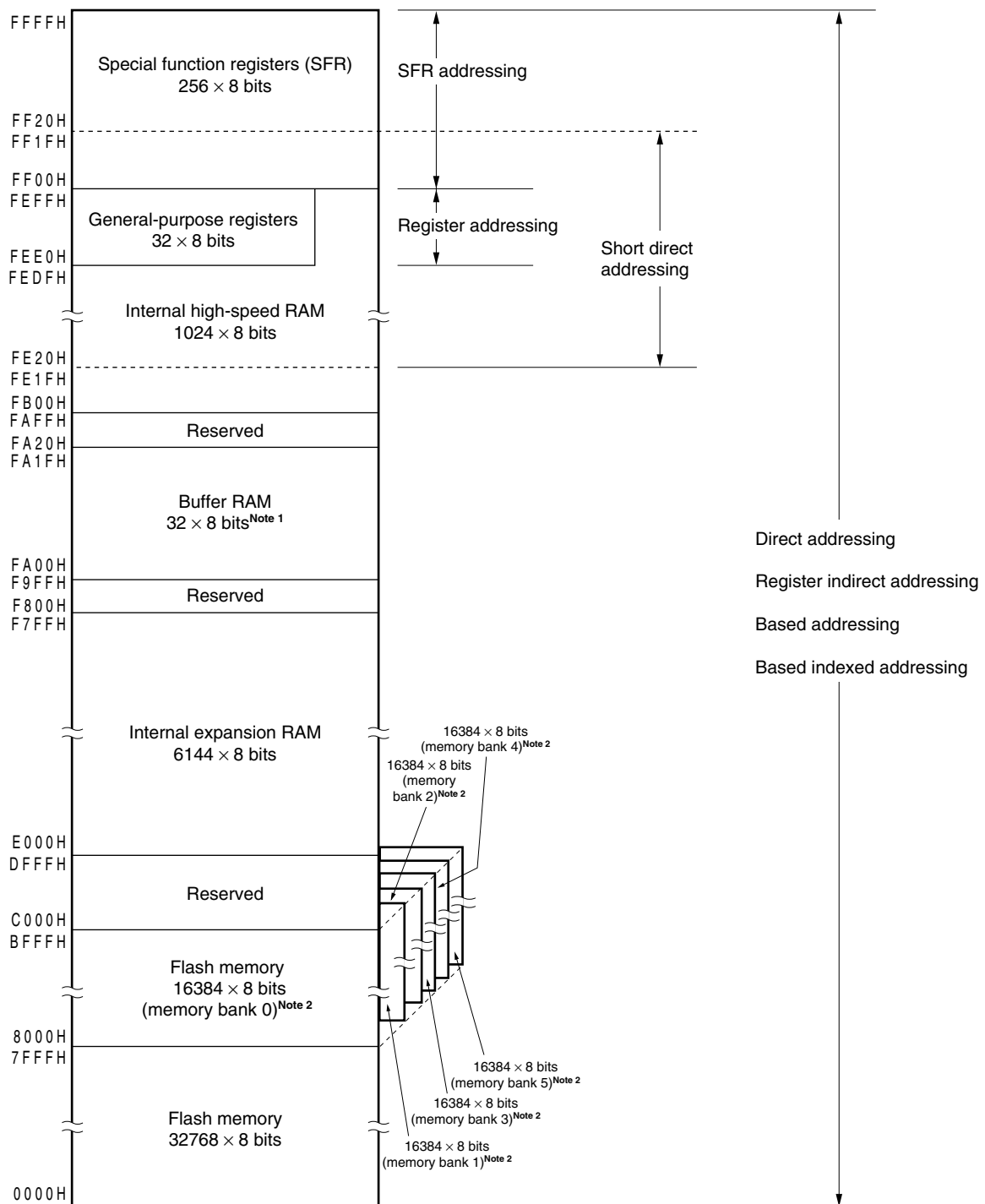
Figure 3-19. Correspondence Between Data Memory and Addressing ( \mu PD78F0527, 78F0527A, 78F0537, 78F0537A, 78F0547, 78F0547A, 78F0527D, 78F0527DA, 78F0537D, 78F0537DA, 78F0547D and 78F0547DA)
