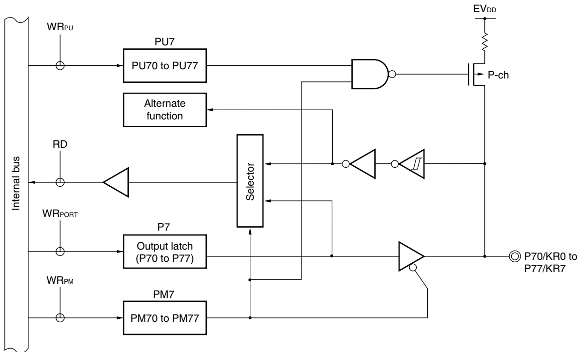
Figure 5-21. Block Diagram of P70 to P77
