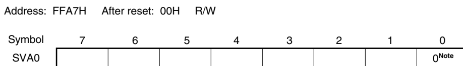
Figure 18-4. Format of Slave Address Register 0 (SVA0)
