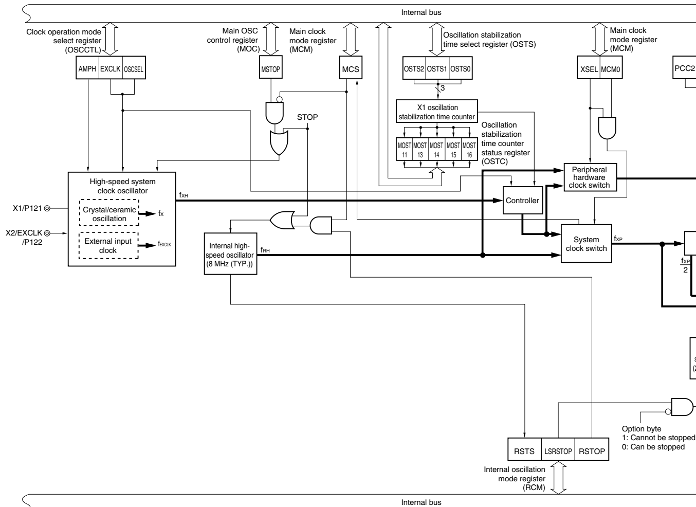
Figure 6-1. Block Diagram of Clock Generator (78K0/KB2)
