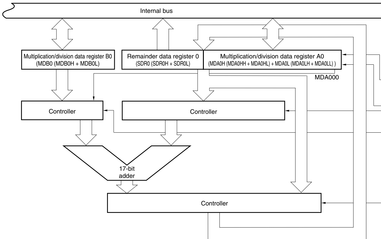
Figure 19-1. Block Diagram of Multiplier/Divider
