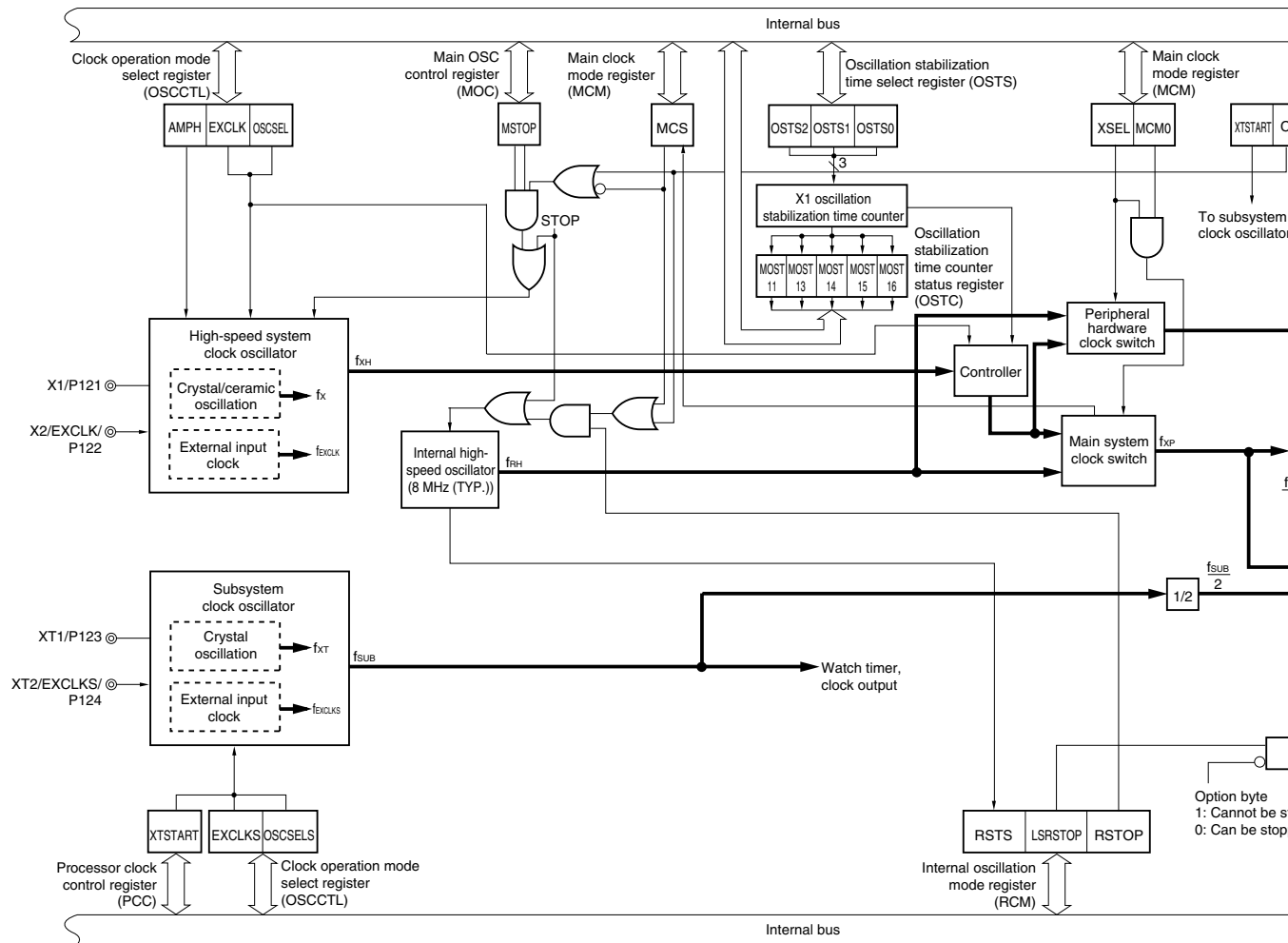
Figure 6-2. Block Diagram of Clock Generator (78K0/KC2, 78K0/KD2, 78K0/KE2, and 78K0/KE2)
