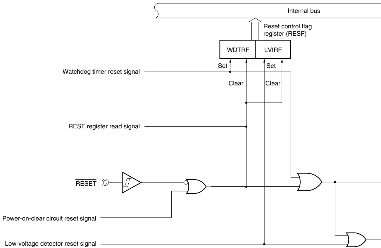
Figure 23-1. Block Diagram of Reset Function
