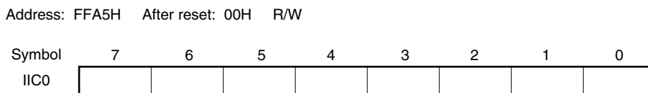
Figure 18-3. Format of IIC Shift Register 0 (IIC0)
