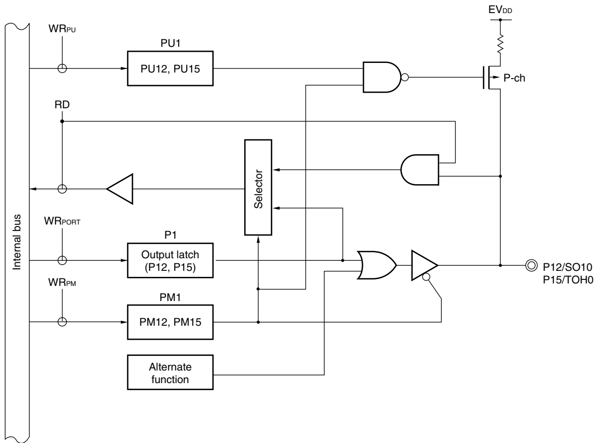
Figure 5-9. Block Diagram of P12 and P15
