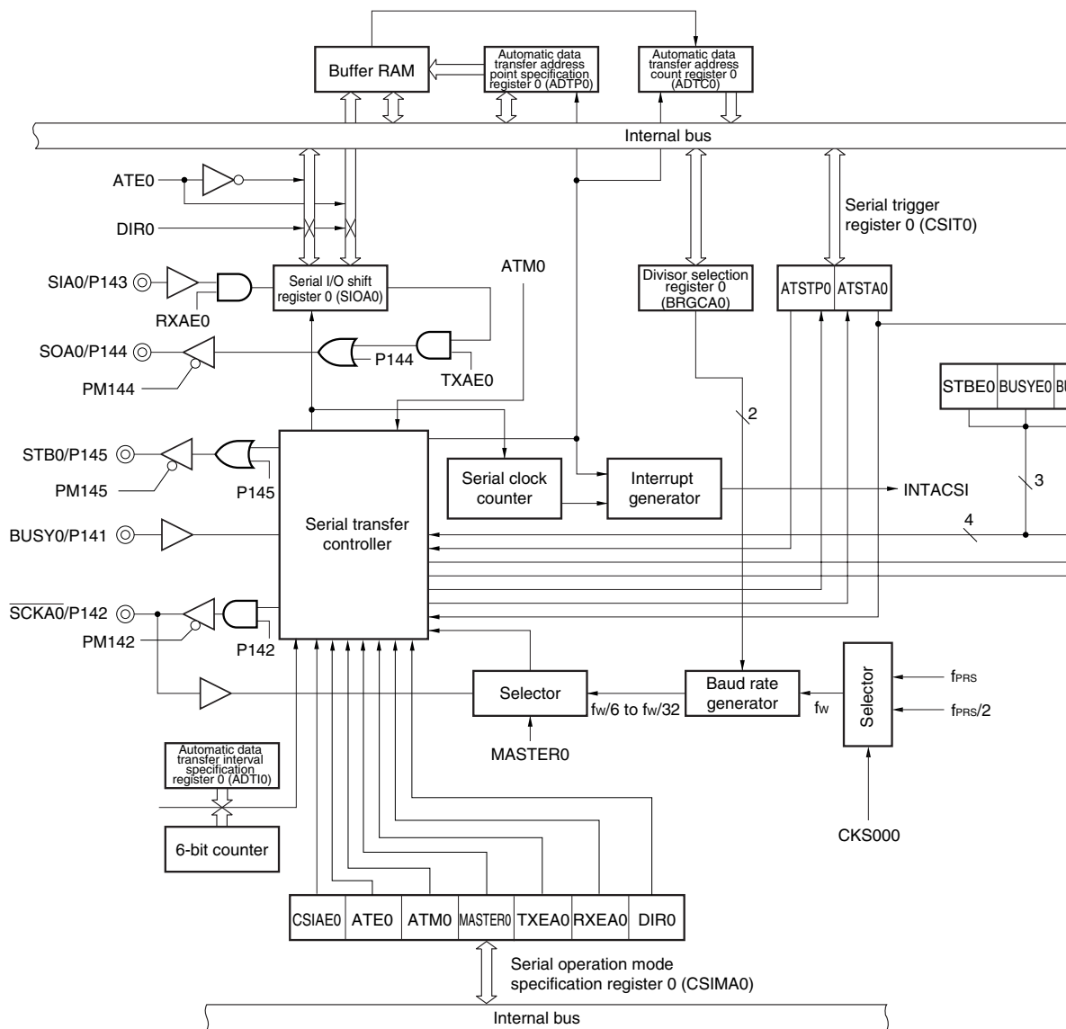
Figure 17-1. Block Diagram of Serial Interface CSIA0
