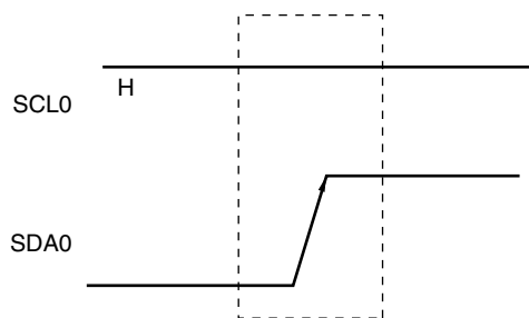
Figure 18-17. Stop Condition
