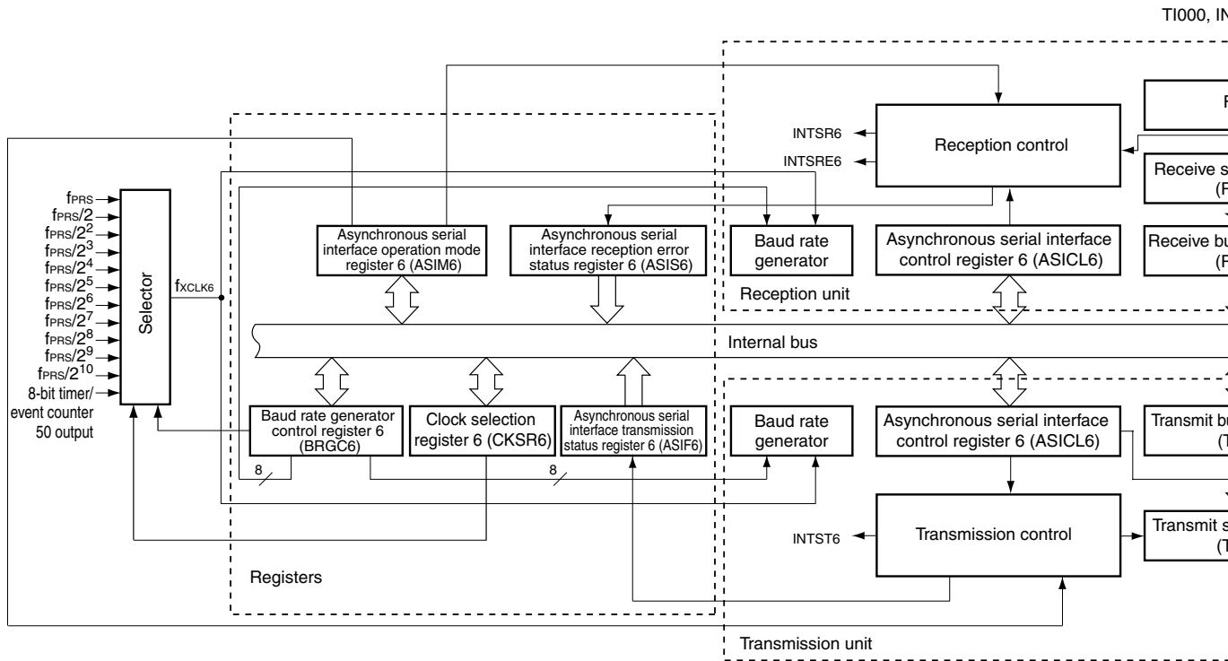
Figure 15-4. Block Diagram of Serial Interface UART6
