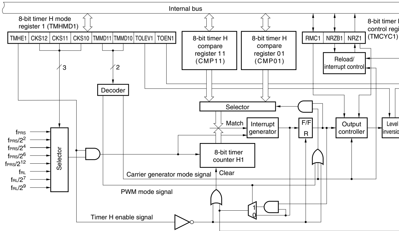
Figure 9-2. Block Diagram of 8-Bit Timer H1
