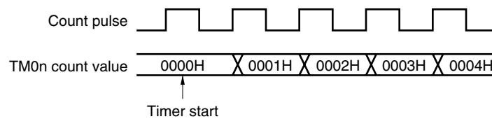
Figure 7-60. Start Timing of TM0n Count
