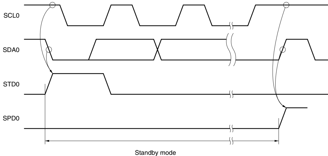
Figure 18-21. Timing for Accepting Communication Reservations
