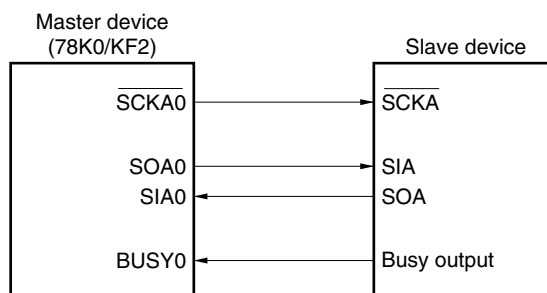
Figure 17-23. System Configuration When Busy Control Option Is Used
