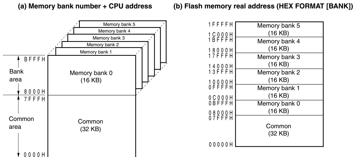
Figure 4-2. Address View
