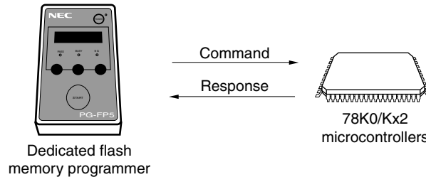
Figure 27-12. Communication Commands
