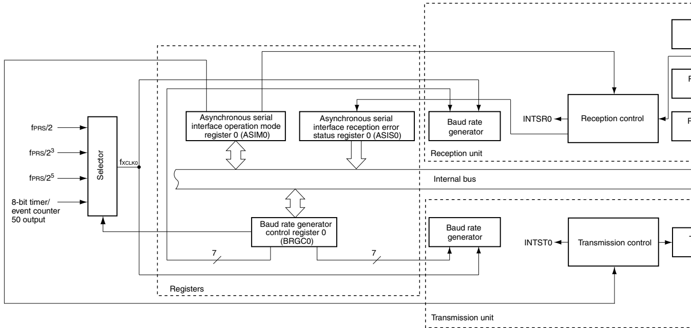
Figure 14-1. Block Diagram of Serial Interface UART0
