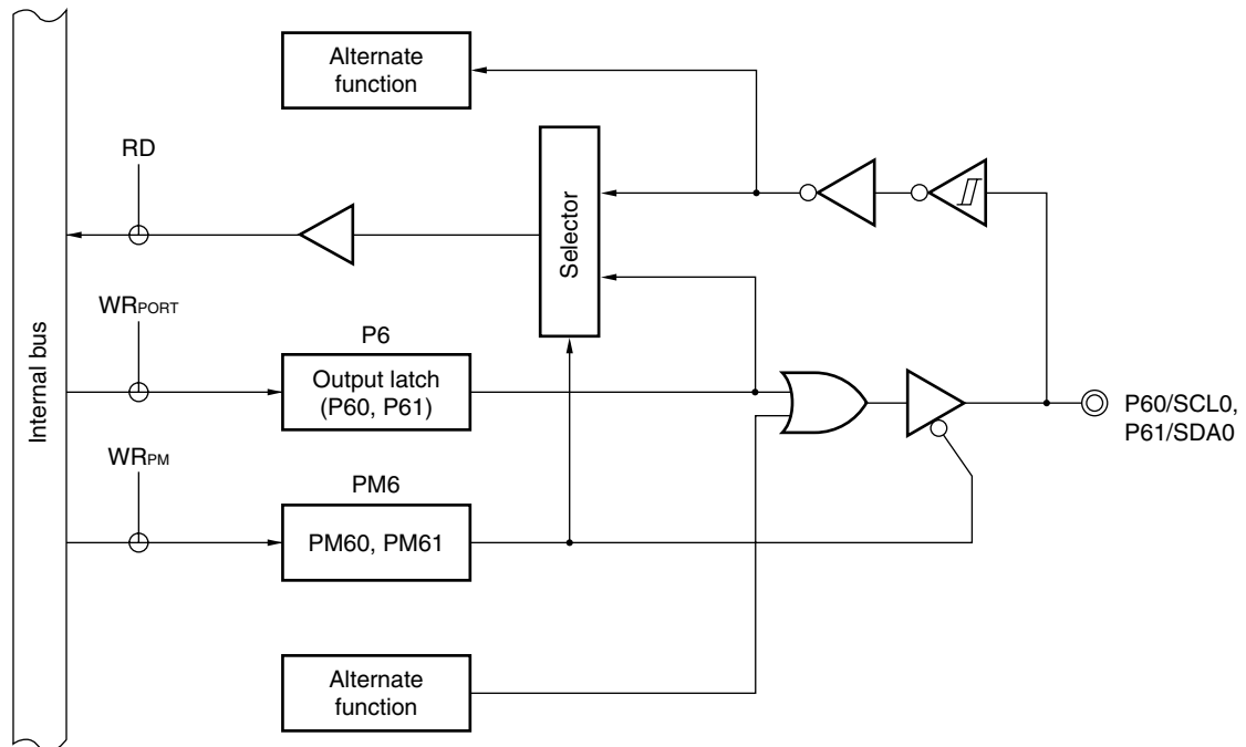
Figure 5-17. Block Diagram of P60 and P61
