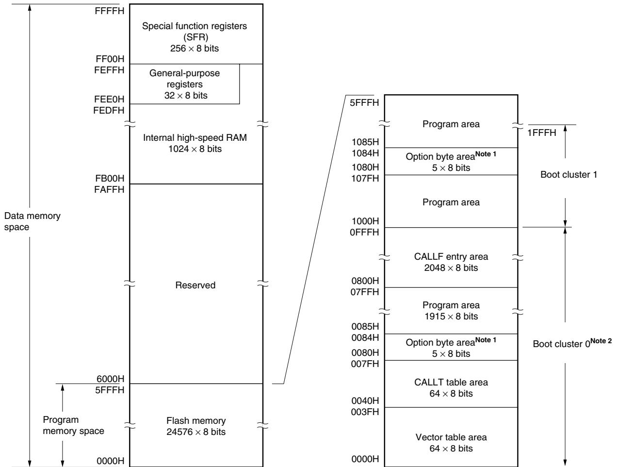
Figure 3-3. Memory Map ( \mu PD78F0502, 78F0502A, 78F0512, 78F0512A, 78F0522, 78F0522A, 78F0532, and 78F0532A)
