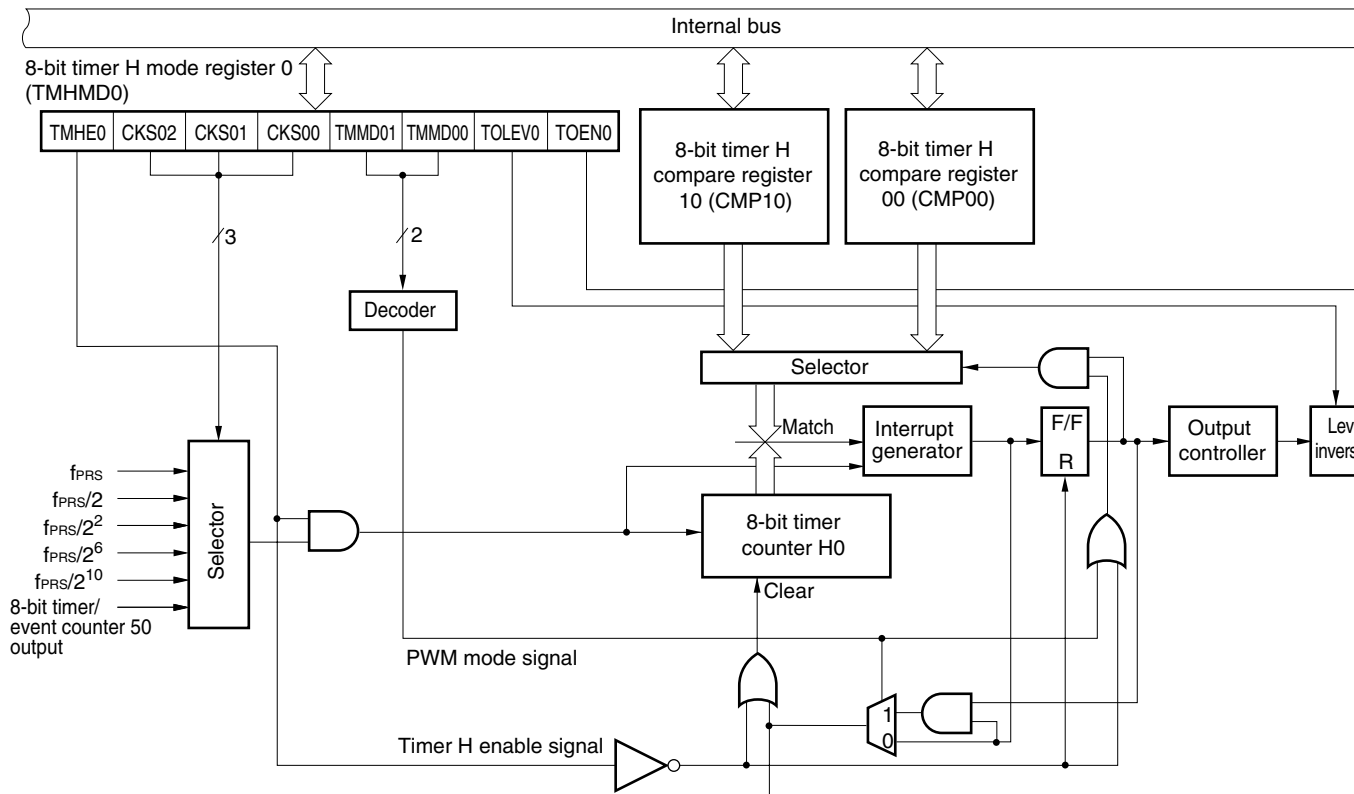
Figure 9-1. Block Diagram of 8-Bit Timer H0
