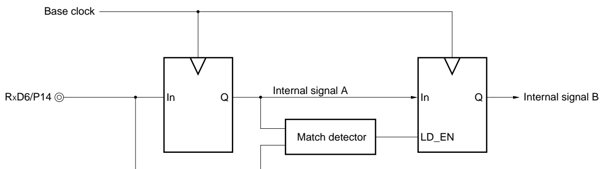
Figure 14-23. Noise Filter Circuit
