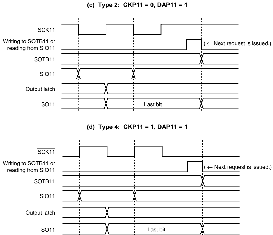
Figure 16-9. Output Value of SO11 Pin (Last Bit) (2/2)
