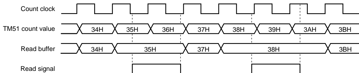
Figure 8-12. 8-bit Timer Counter 51 (TM51) Read Timing
