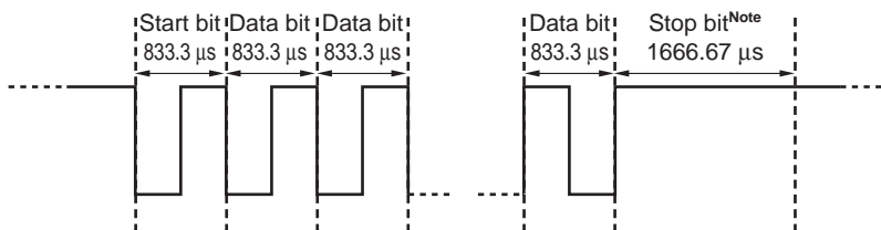
Figure 14-29. Timing in the Frame
