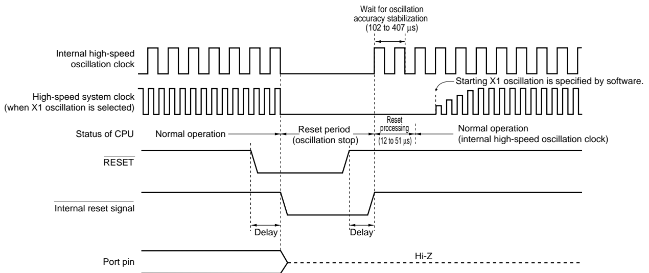
Figure 20-2. Timing of Reset by \overline{\text{RESET}} Input
