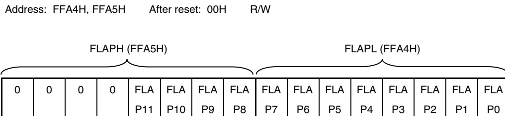
Figure 16-14. Format of Flash Address Pointer H/L (FLAPH/FLAPL)
