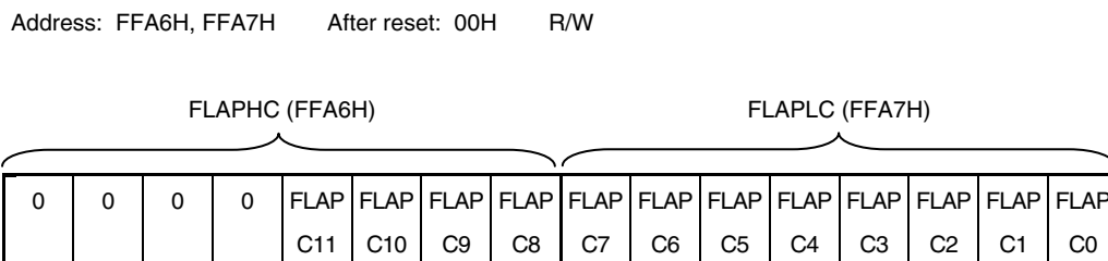
Figure 16-15. Format of Flash Address Pointer H/L Compare Registers (FLAPHC/FLAPLC)
