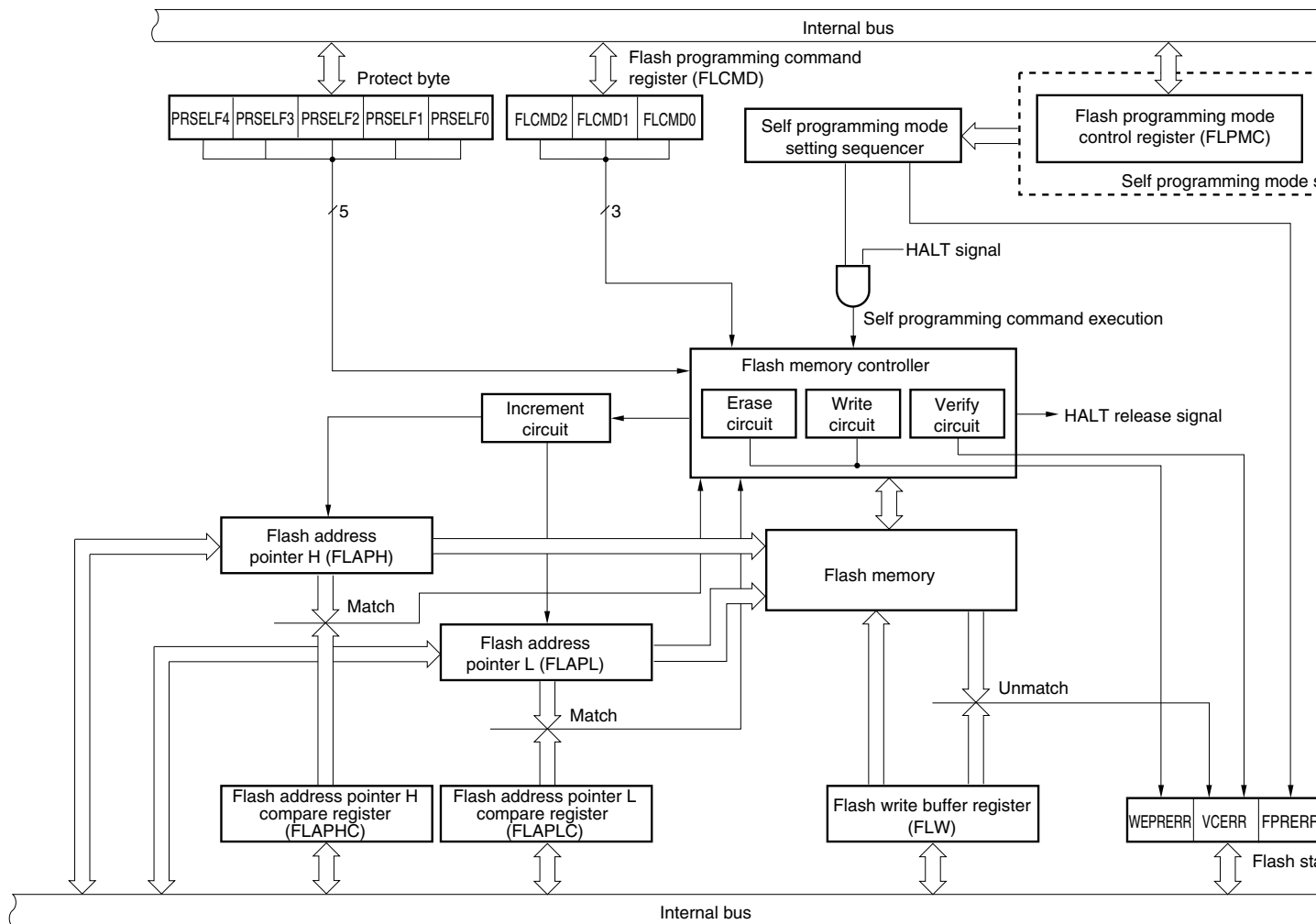
Figure 16-8. Block Diagram of Self Programming
