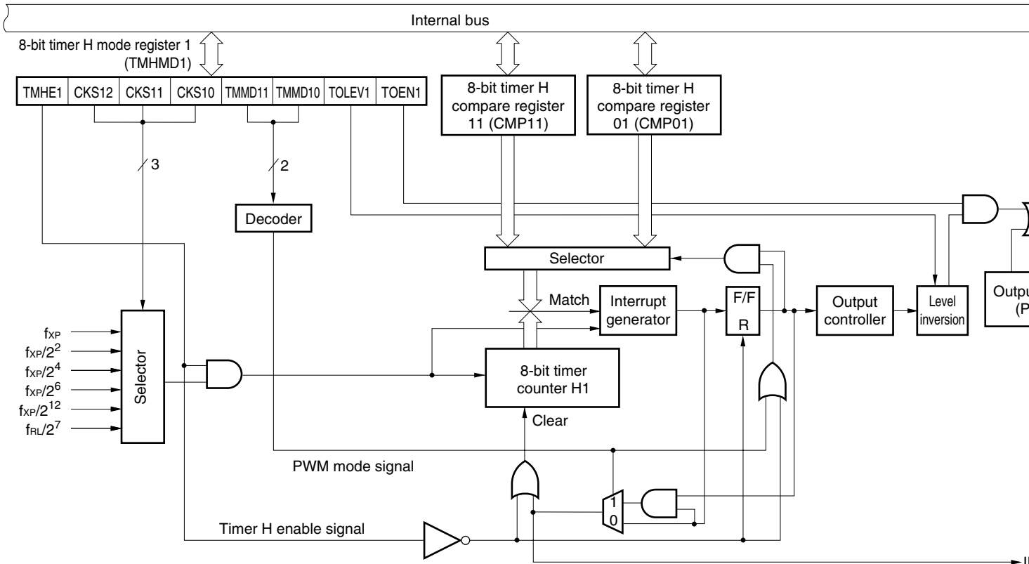
Figure 7-1. Block Diagram of 8-Bit Timer H1
