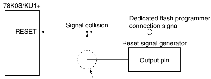
Figure 16-6. Signal Collision ( \overline{\text{RESET}} Pin)
