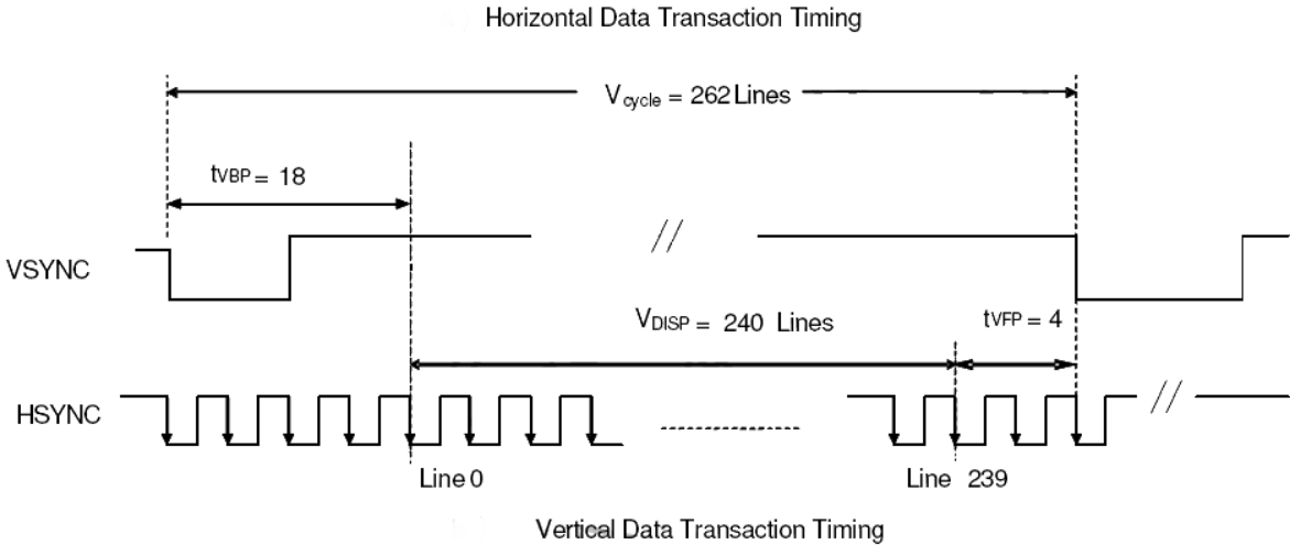
Figure 3. Data Transaction Timing in Parallel RGB (24 bit) Interface (SYNC Mode)
